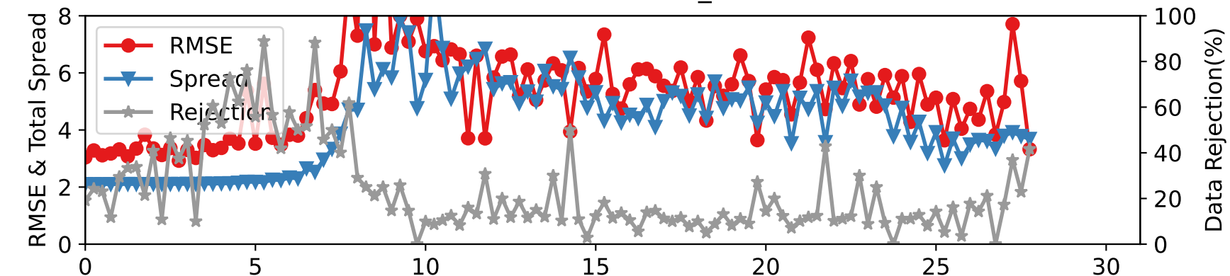
DARTEN10 — RADIOSONDE_U at 2-15 hPa
