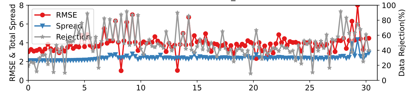
DARTEN40 — RADIOSONDE_U at 2-15 hPa
