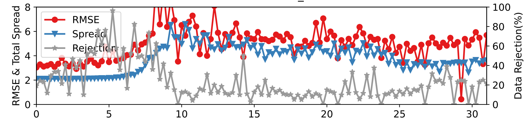
DARTEN20 — RADIOSONDE_U at 2-15 hPa
