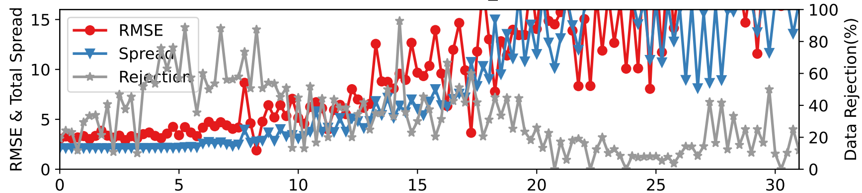
CTRLN10 — RADIOSONDE_U at 2-15 hPa
