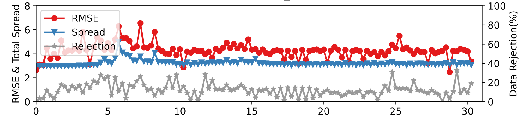
DARTEN40 — RADIOSONDE_U at 275-350 hPa
