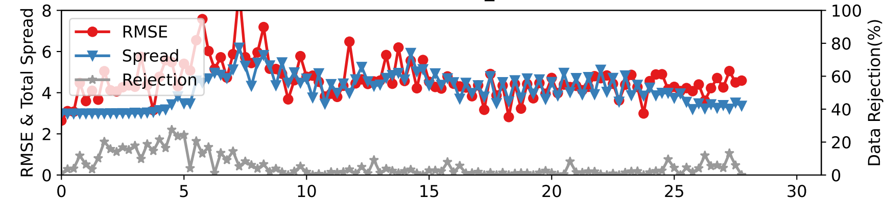
DARTEN10 — RADIOSONDE_U at 275-350 hPa
