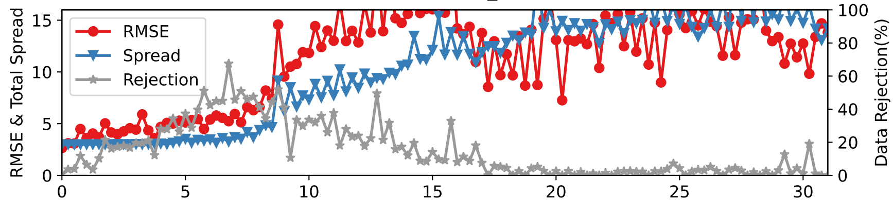
CTRLN10 — RADIOSONDE_U at 275-350 hPa
