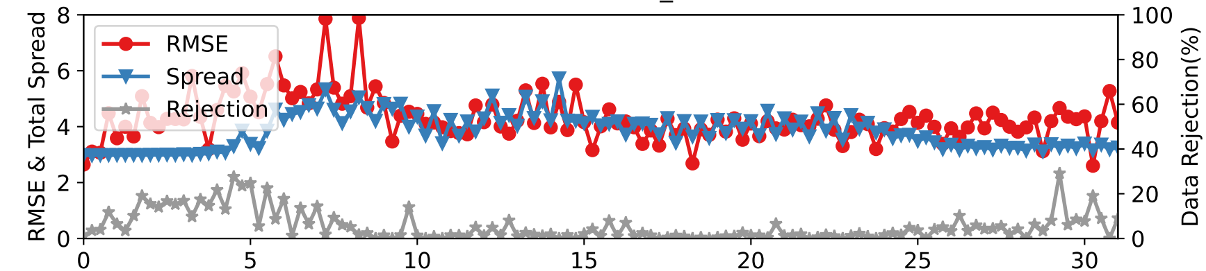
DARTEN20 — RADIOSONDE_U at 275-350 hPa
