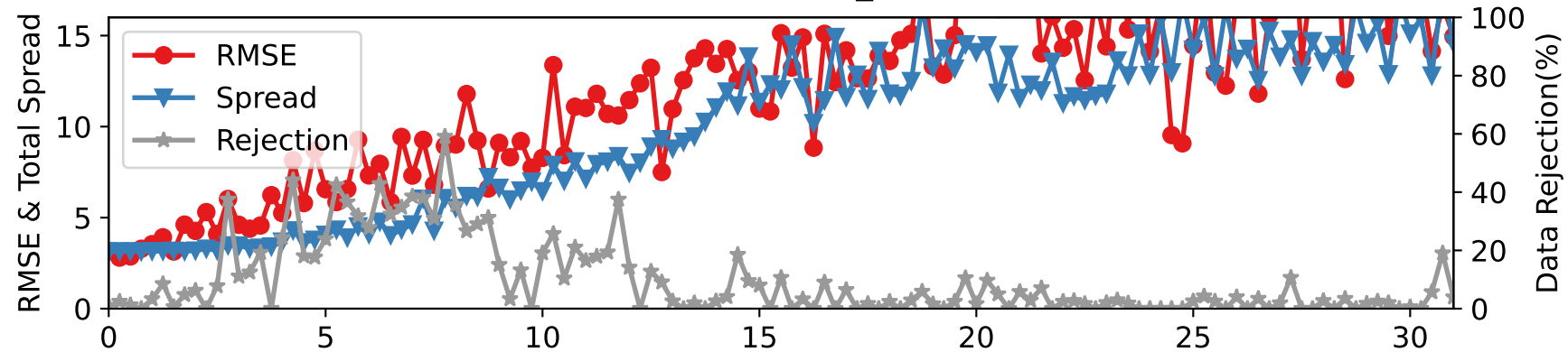
CTRLN10 — RADIOSONDE_U at 225-275 hPa
