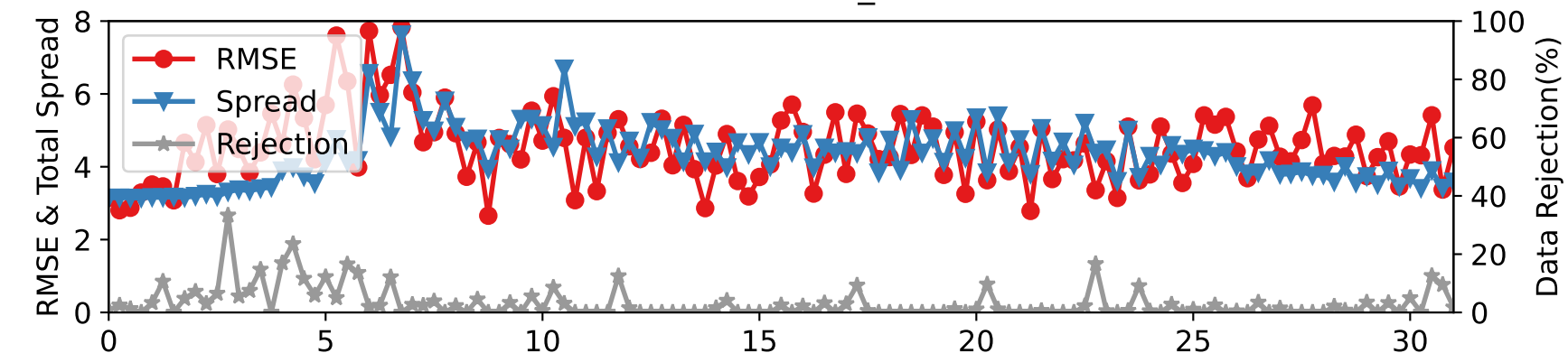
DARTEN20 — RADIOSONDE_U at 225-275 hPa
