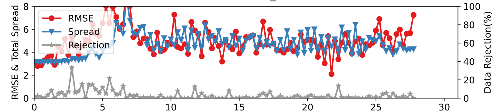
DARTEN10 — RADIOSONDE_U at 225-275 hPa
