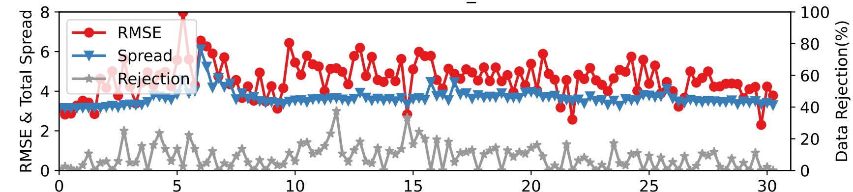
DARTEN40 — RADIOSONDE_U at 225-275 hPa
