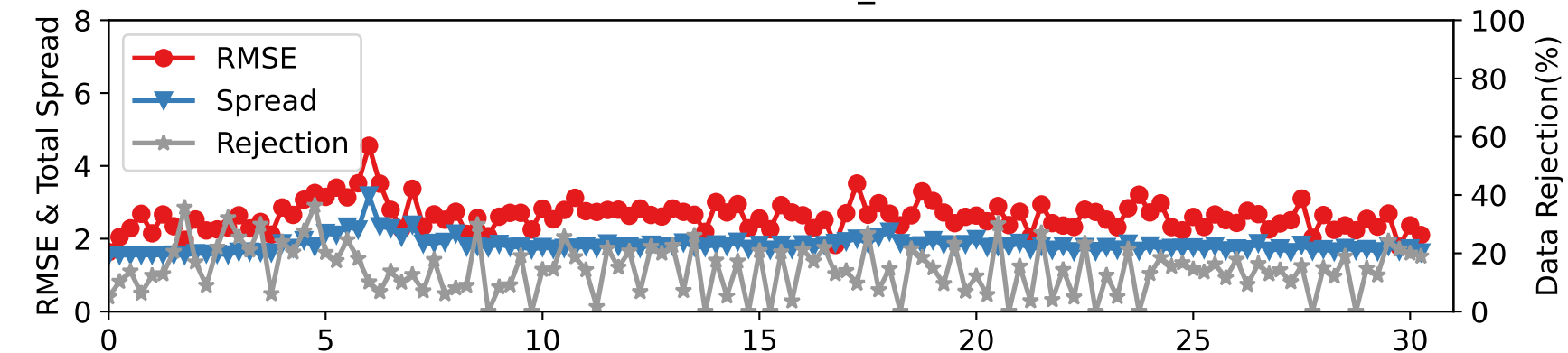
DARTEN40 — RADIOSONDE_U at 775-887 hPa
