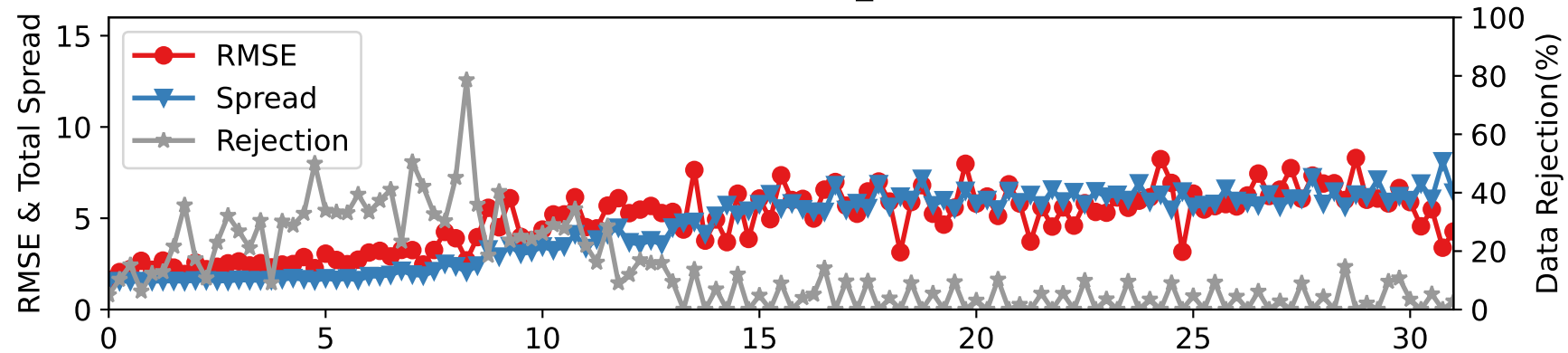
CTRLN10 — RADIOSONDE_U at 775-887 hPa
