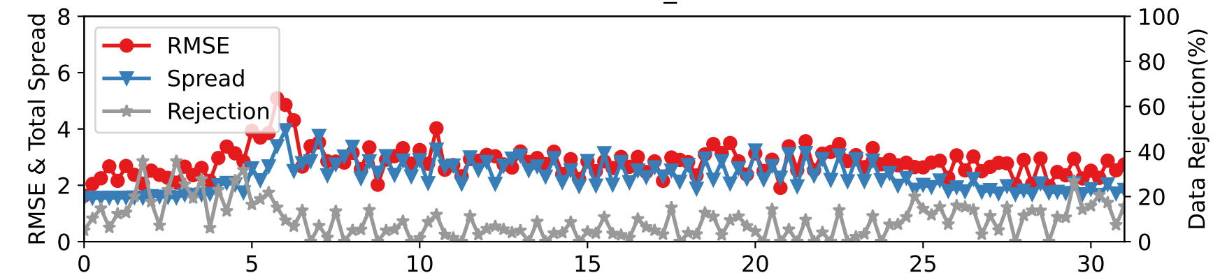
DARTEN20 — RADIOSONDE_U at 775-887 hPa
