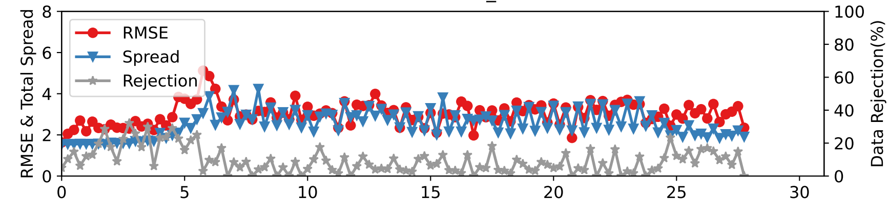
DARTEN10 — RADIOSONDE_U at 775-887 hPa
