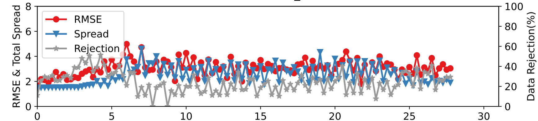
DARTEN10 — RADIOSONDE_U at 887-962 hPa
