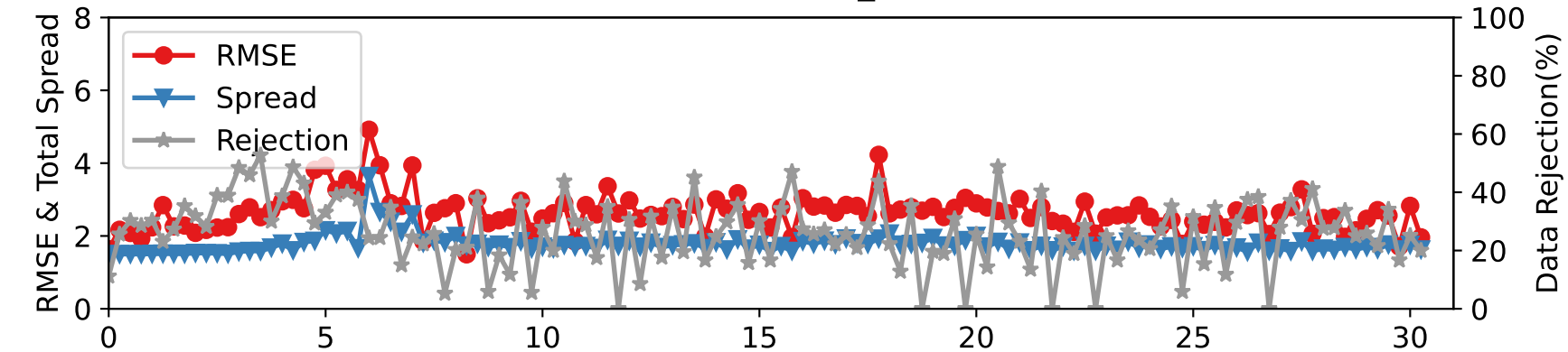
DARTEN40 — RADIOSONDE_U at 887-962 hPa
