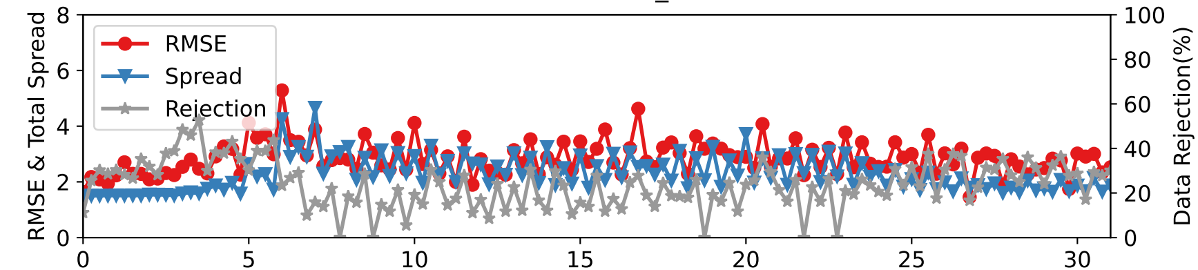
DARTEN20 — RADIOSONDE_U at 887-962 hPa
