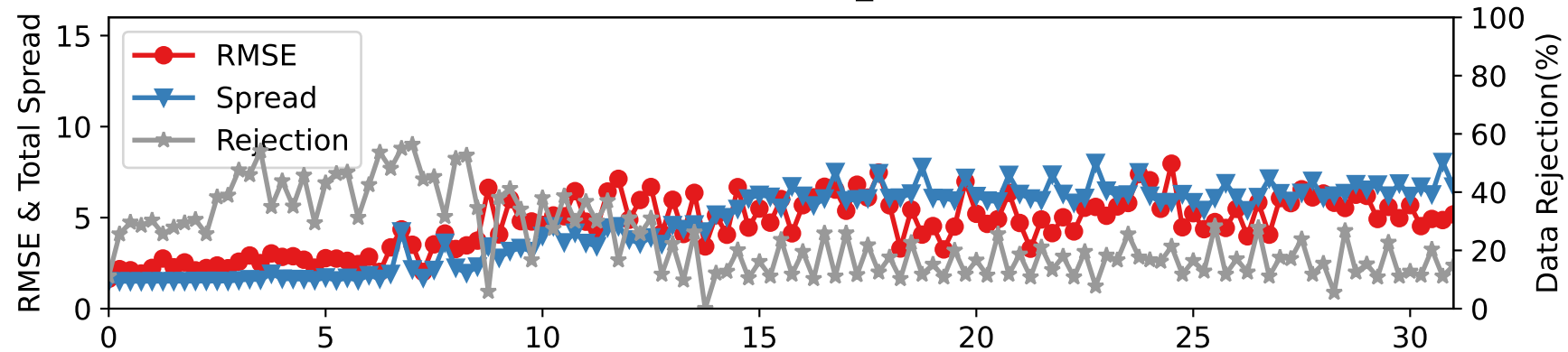
CTRLN10 — RADIOSONDE_U at 887-962 hPa
