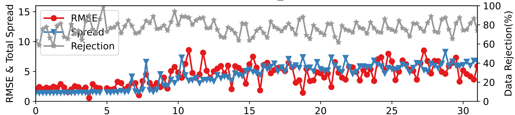
CTRLN10 — RADIOSONDE_U at 962-1035 hPa
