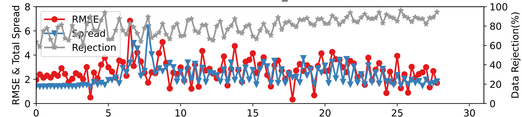
DARTEN10 — RADIOSONDE_U at 962-1035 hPa
