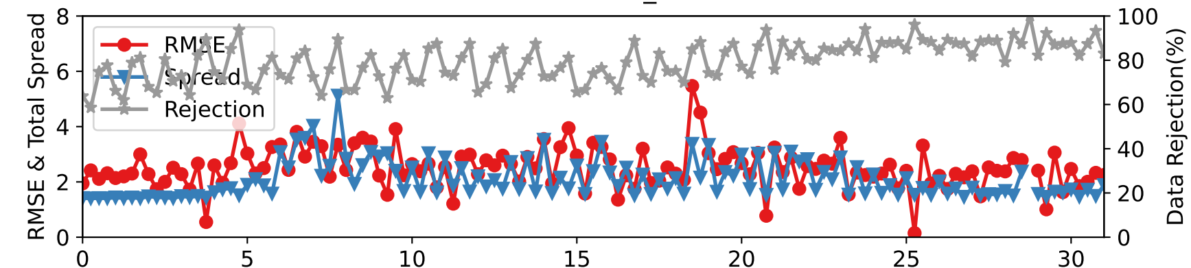
DARTEN20 — RADIOSONDE_U at 962-1035 hPa
