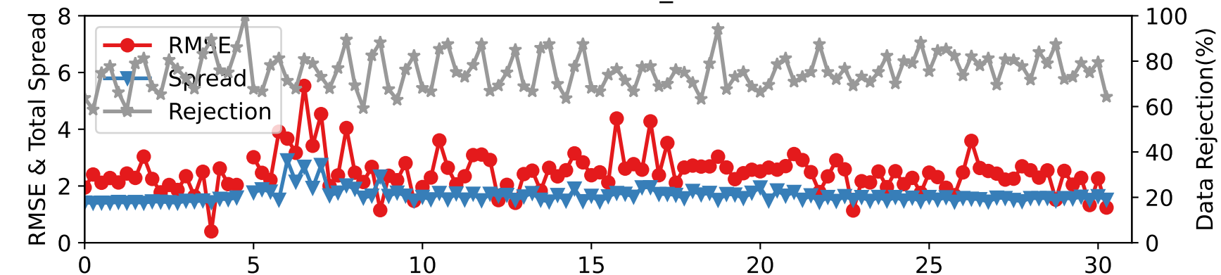
DARTEN40 — RADIOSONDE_U at 962-1035 hPa
