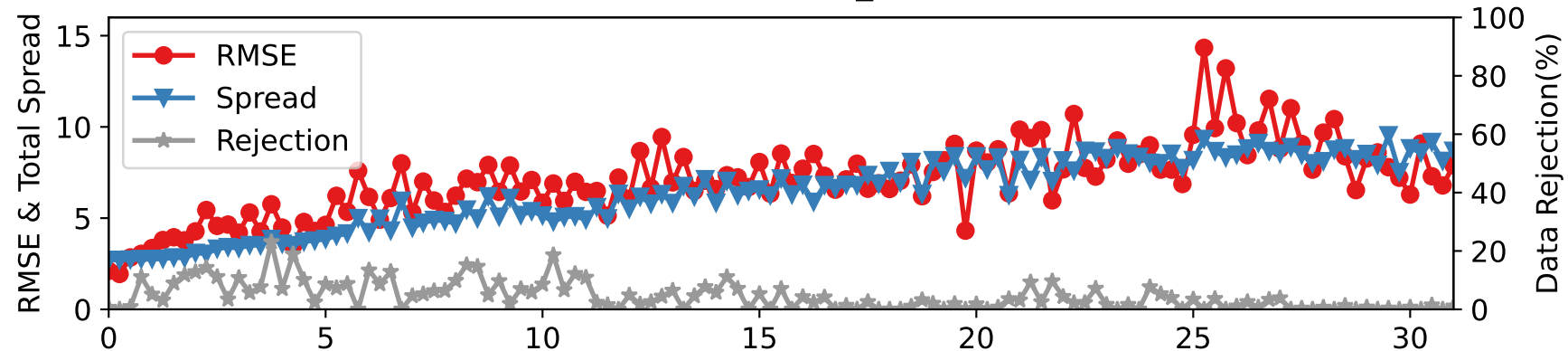
CTRLN10 — RADIOSONDE_U at 175-225 hPa
