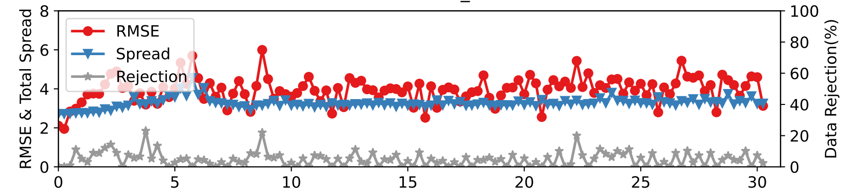
DARTEN40 — RADIOSONDE_U at 175-225 hPa
