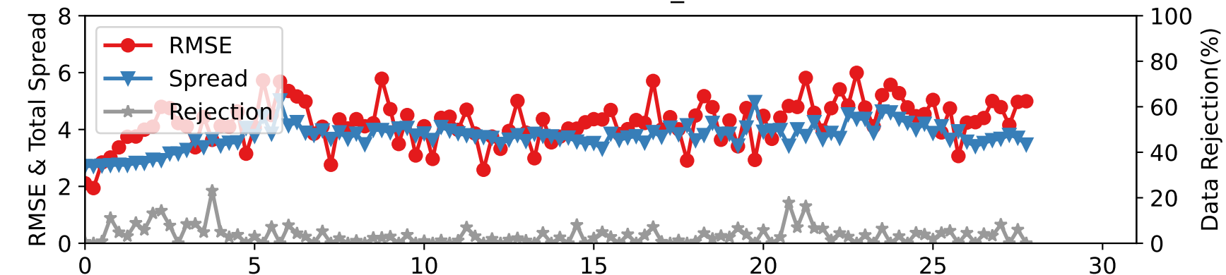
DARTEN10 — RADIOSONDE_U at 175-225 hPa
