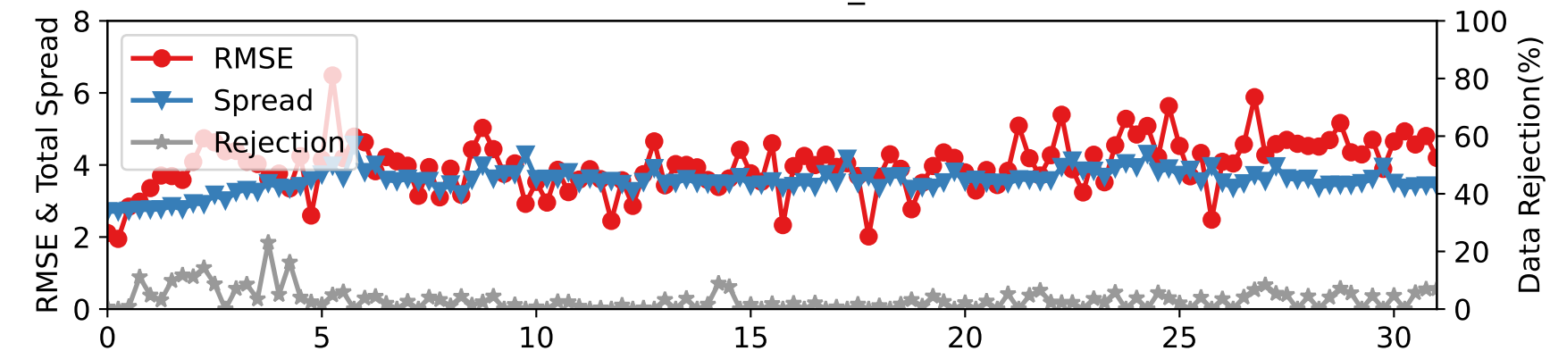
DARTEN20 — RADIOSONDE_U at 175-225 hPa
