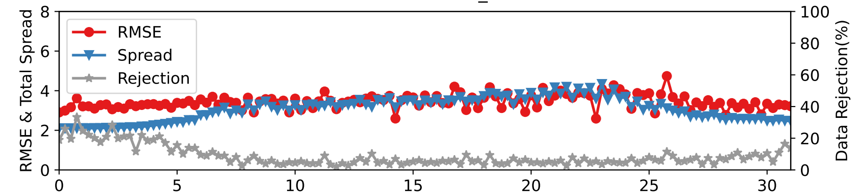
DARTEN20 — RADIOSONDE_U at 35-75 hPa
