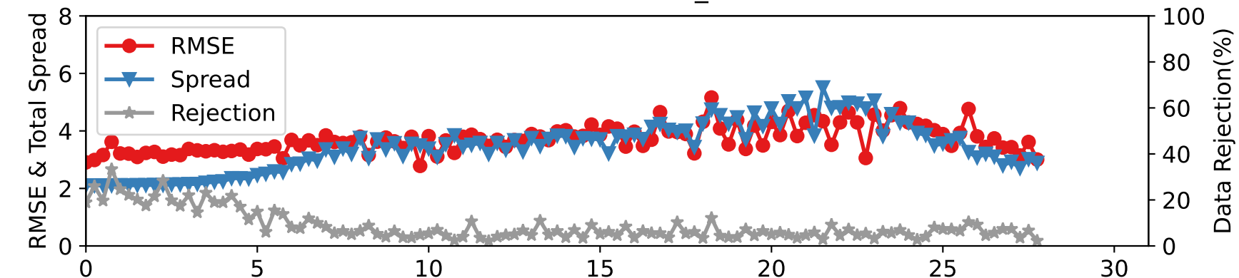
DARTEN10 — RADIOSONDE_U at 35-75 hPa
