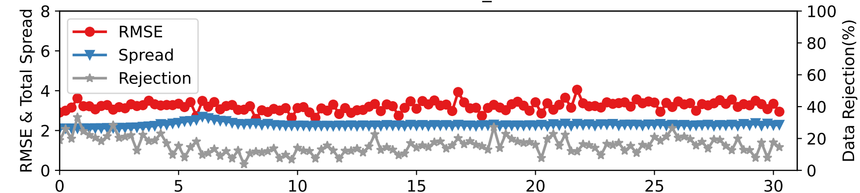
DARTEN40 — RADIOSONDE_U at 35-75 hPa
