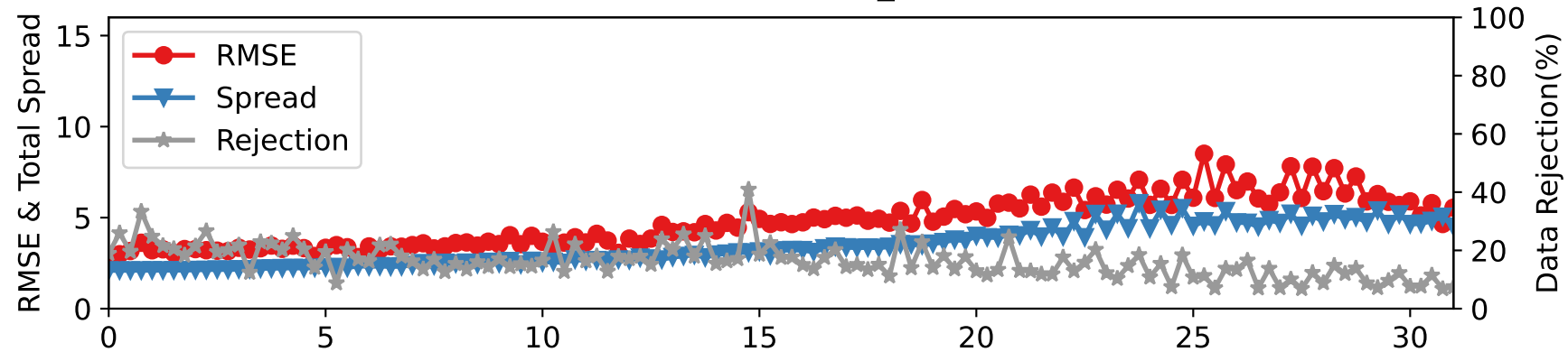
CTRLN10 — RADIOSONDE_U at 35-75 hPa
