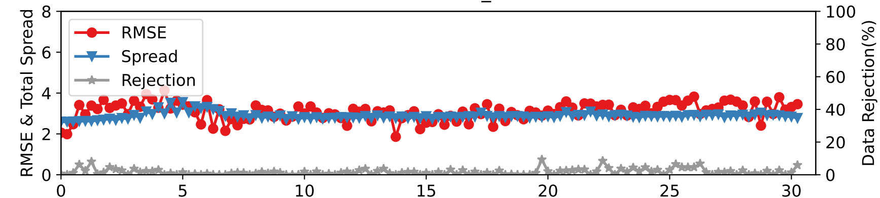
DARTEN40 — RADIOSONDE_U at 350-450 hPa
