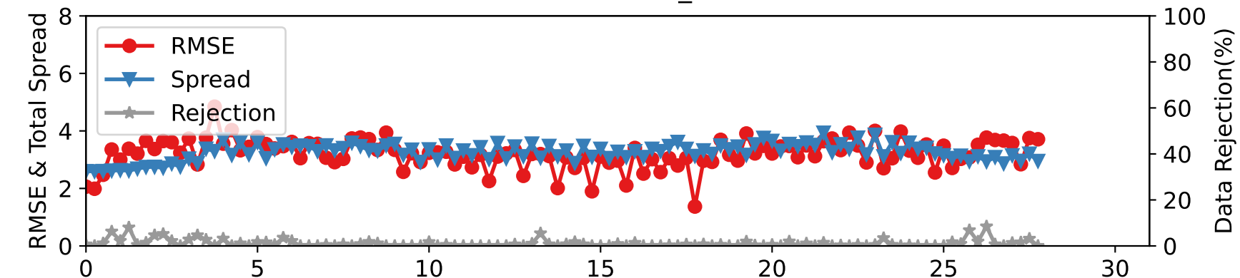
DARTEN10 — RADIOSONDE_U at 350-450 hPa
