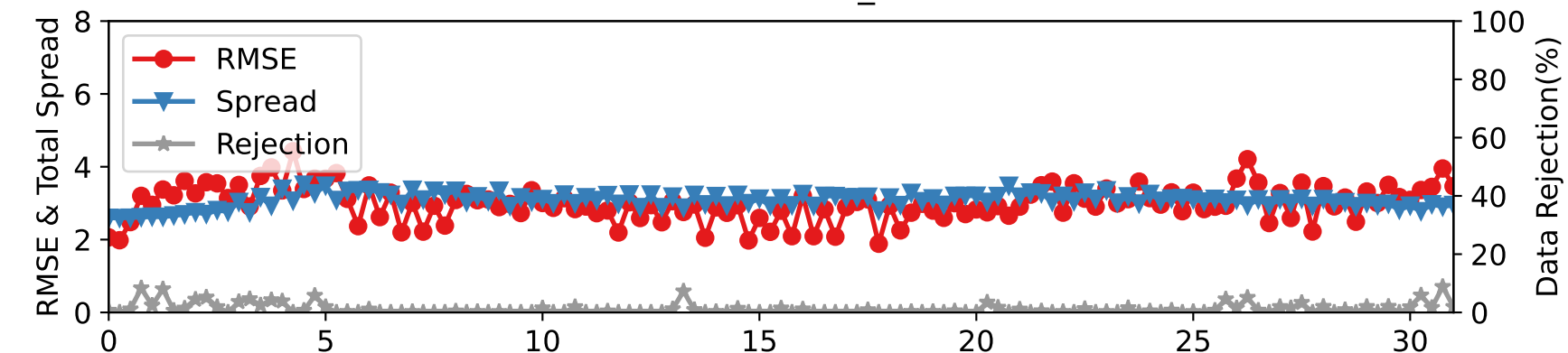
DARTEN20 — RADIOSONDE_U at 350-450 hPa
