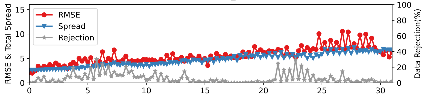
CTRLN10 — RADIOSONDE_U at 350-450 hPa
