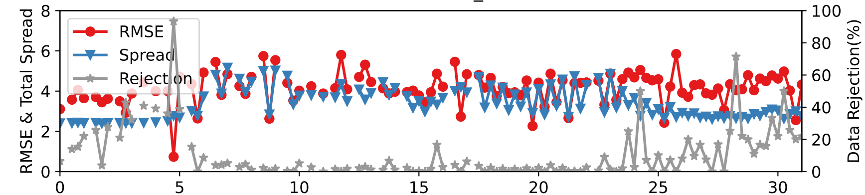
DARTEN20 — RADIOSONDE_V at 125-175 hPa
