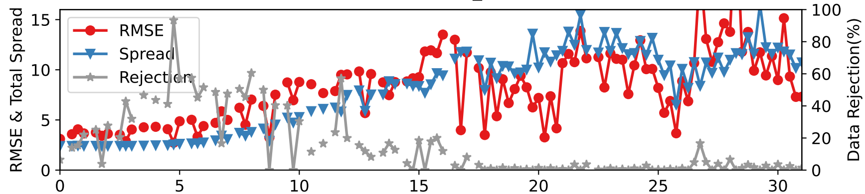
CTRLN10 — RADIOSONDE_V at 125-175 hPa
