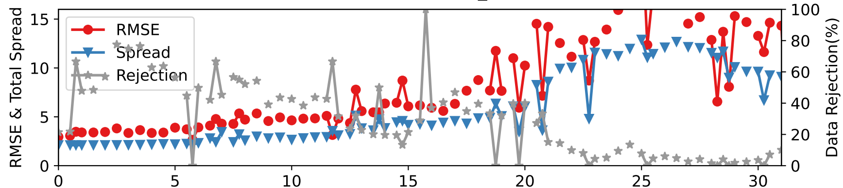
CTRLN10 — RADIOSONDE_V at 2-15 hPa
