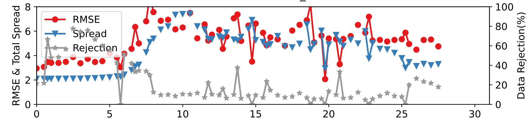
DARTEN10 — RADIOSONDE_V at 2-15 hPa
