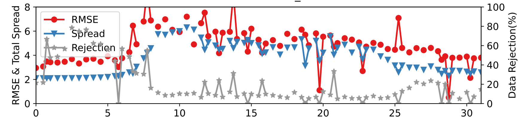
DARTEN20 — RADIOSONDE_V at 2-15 hPa
