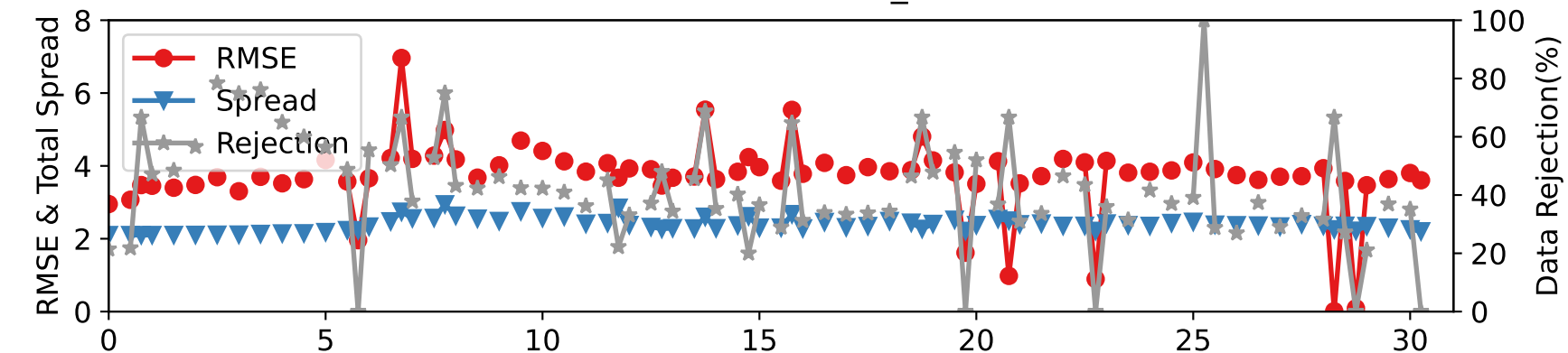
DARTEN40 — RADIOSONDE_V at 2-15 hPa
