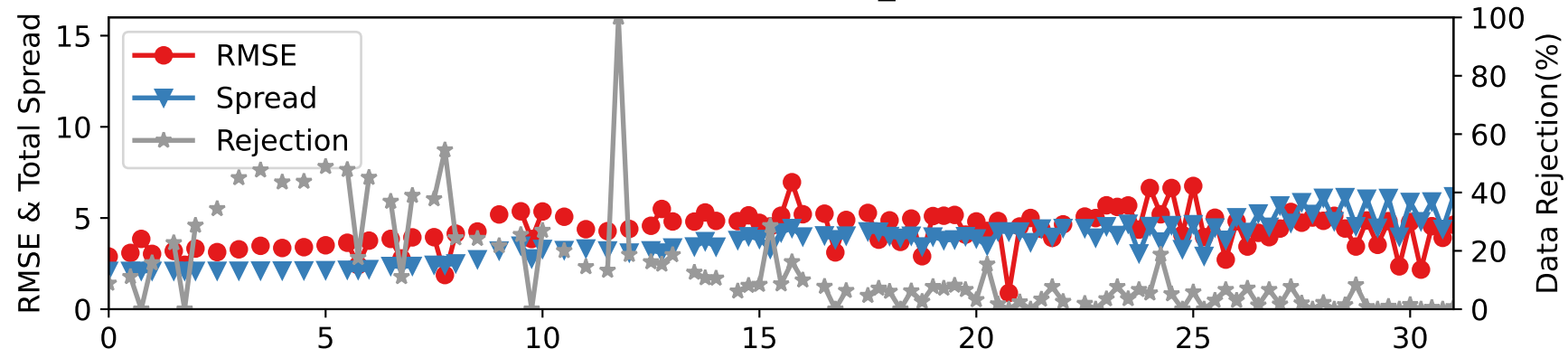
CTRLN10 — RADIOSONDE_V at 35-75 hPa
