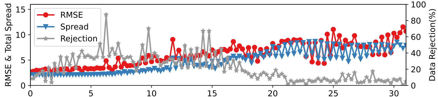
CTRLN10 — RADIOSONDE_V at 15-35 hPa
