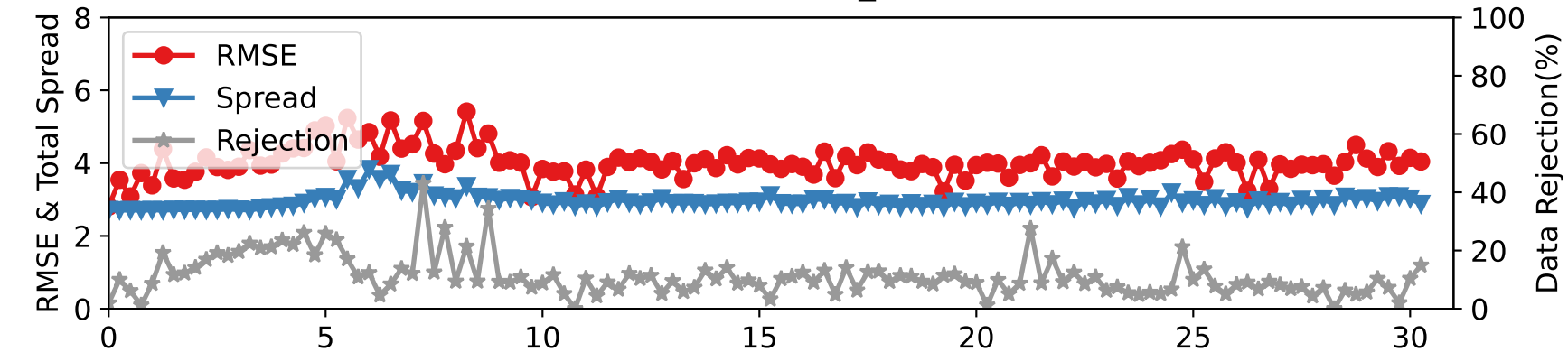
DARTEN40 — RADIOSONDE_V at 175-225 hPa
