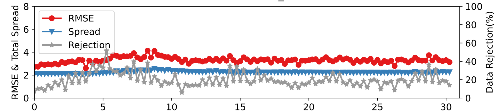
DARTEN40 — RADIOSONDE_V at 35-75 hPa
