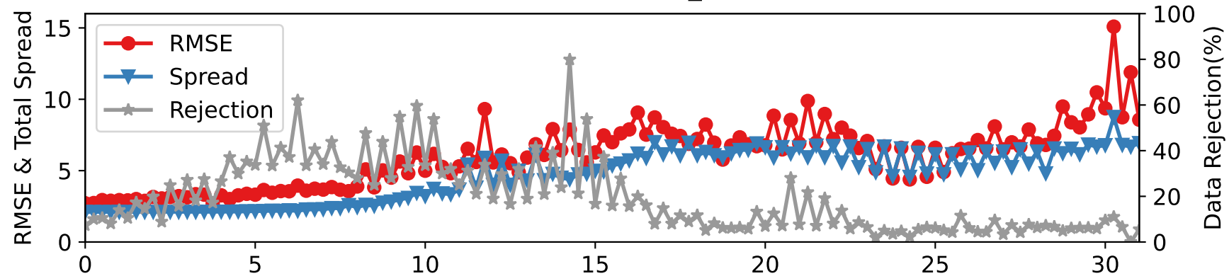
CTRLN10 — RADIOSONDE_V at 35-75 hPa
