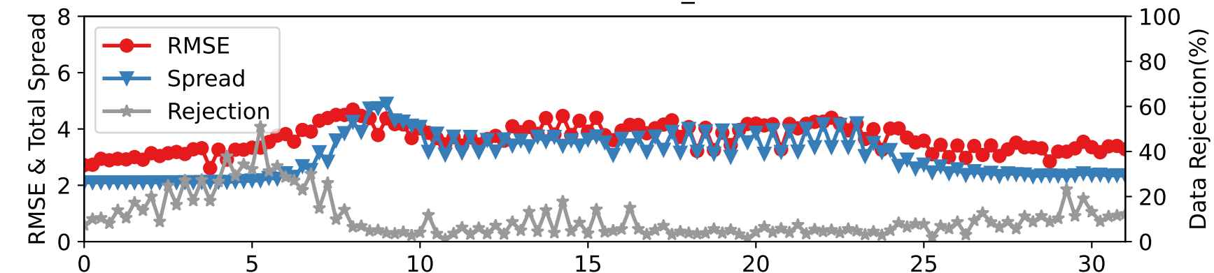
DARTEN20 — RADIOSONDE_V at 35-75 hPa
