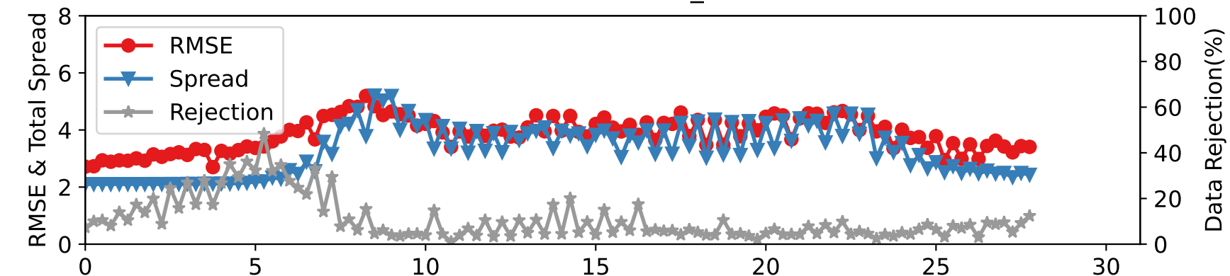
DARTEN10 — RADIOSONDE_V at 35-75 hPa
