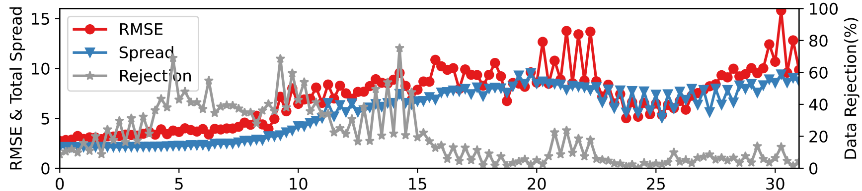
CTRLN10 — RADIOSONDE_V at 75-125 hPa
