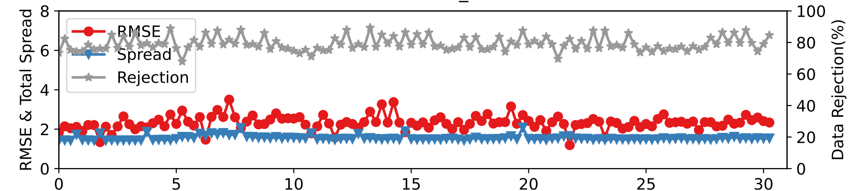
DARTEN40 — RADIOSONDE_V at 962-1035 hPa
