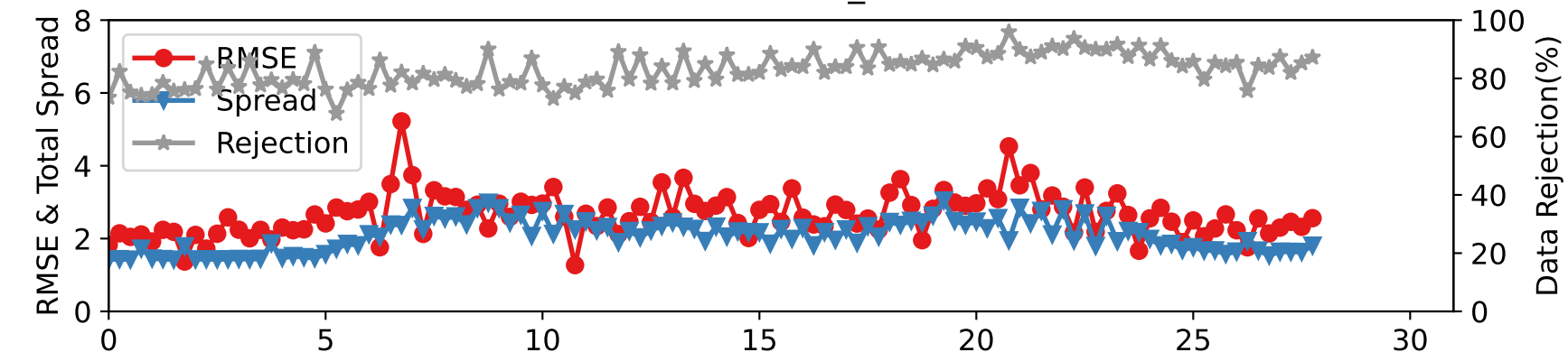
DARTEN10 — RADIOSONDE_V at 962-1035 hPa
