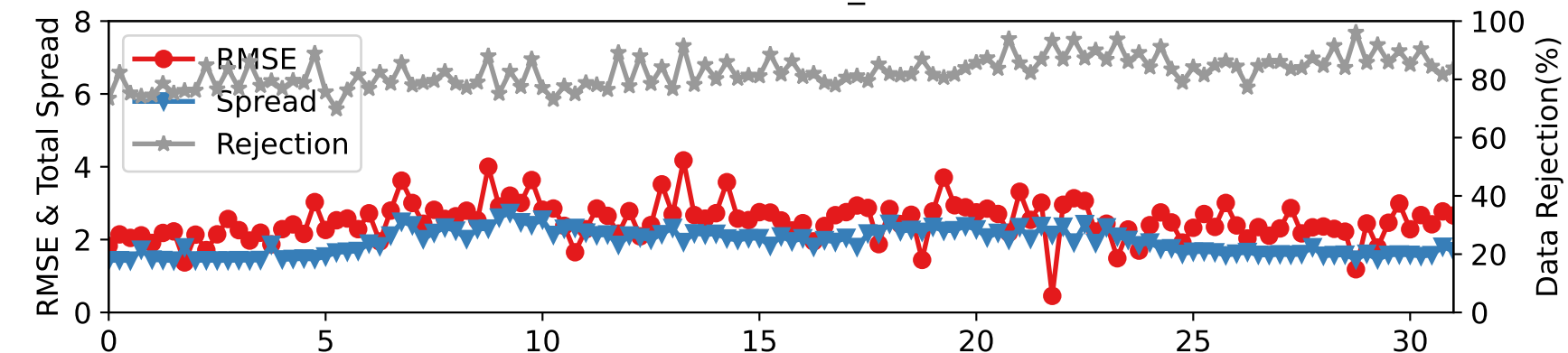
DARTEN20 — RADIOSONDE_V at 962-1035 hPa
