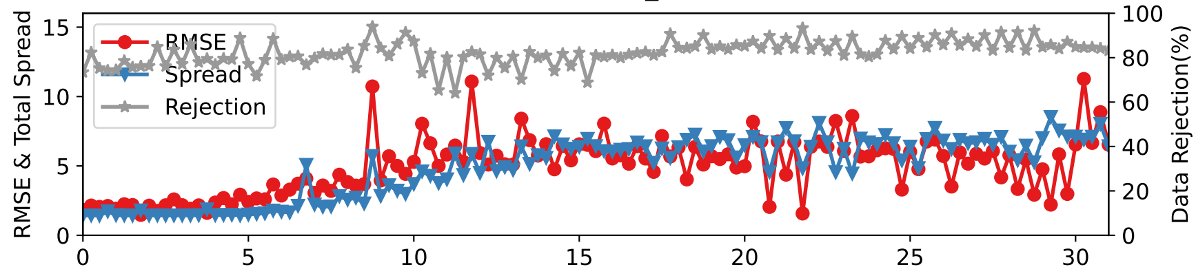
CTRLN10 — RADIOSONDE_V at 962-1035 hPa
