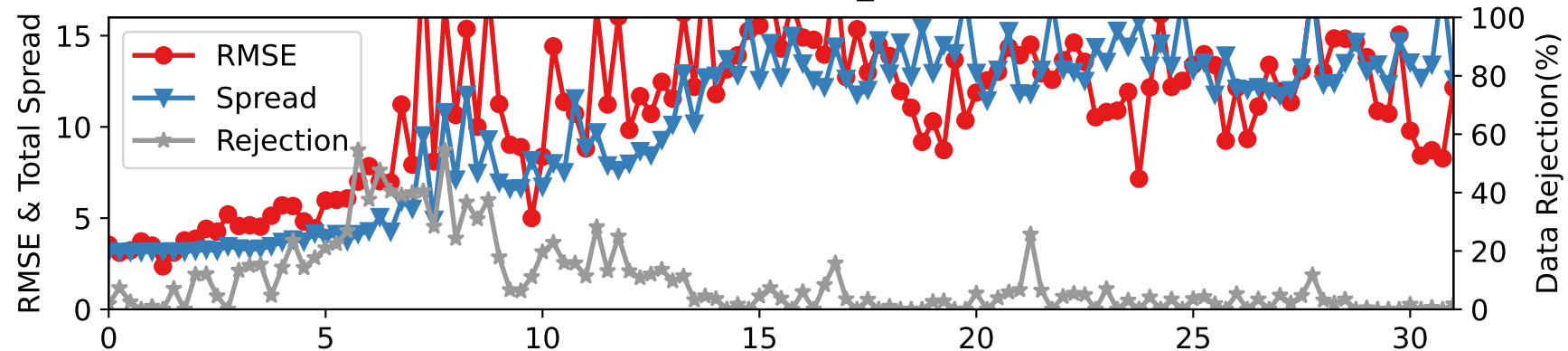
CTRLN10 — RADIOSONDE_V at 225-275 hPa
