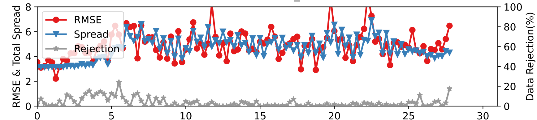
DARTEN10 — RADIOSONDE_V at 225-275 hPa
