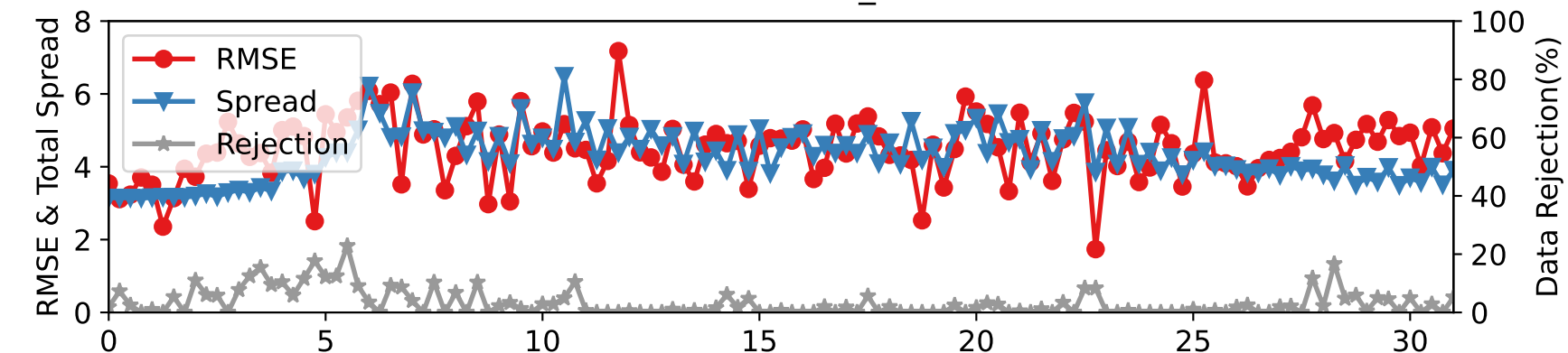
DARTEN20 — RADIOSONDE_V at 225-275 hPa
