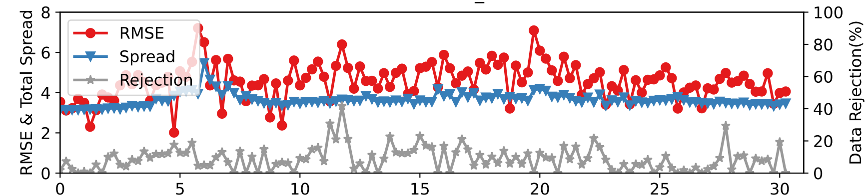
DARTEN40 — RADIOSONDE_V at 225-275 hPa
