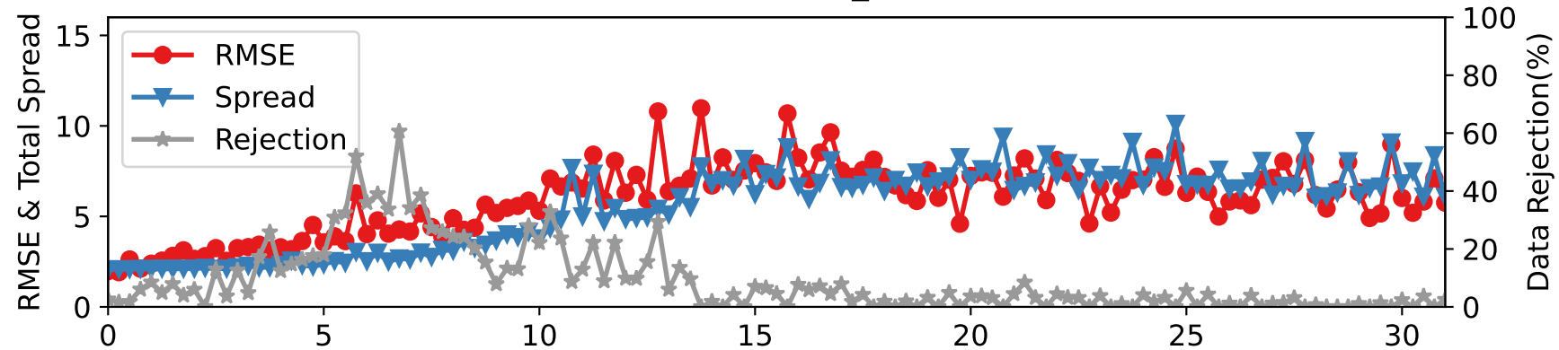
CTRLN10 — RADIOSONDE_V at 450-600 hPa
