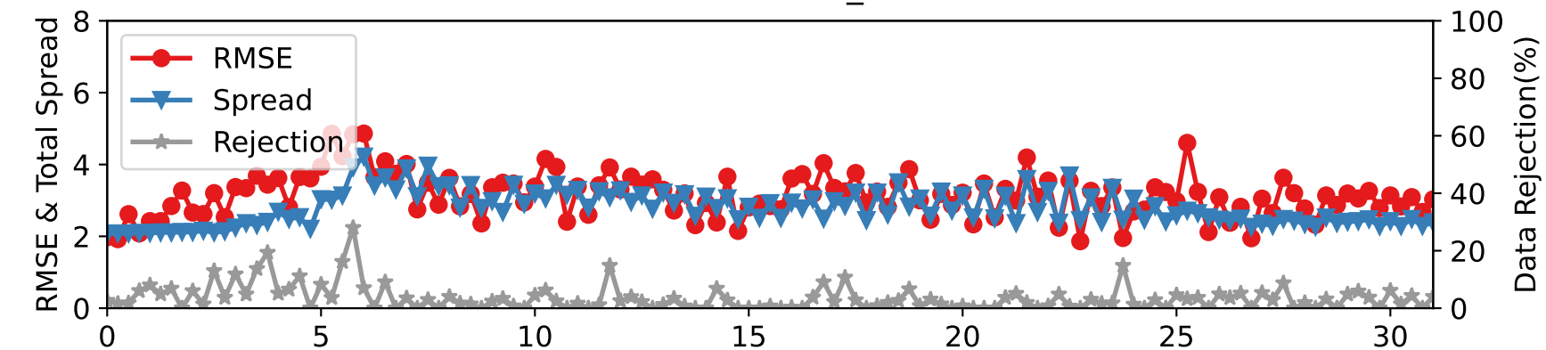
DARTEN20 — RADIOSONDE_V at 450-600 hPa
