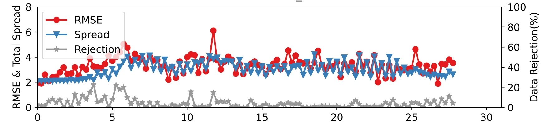
DARTEN10 — RADIOSONDE_V at 450-600 hPa
