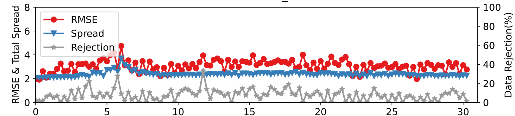
DARTEN40 — RADIOSONDE_V at 450-600 hPa
