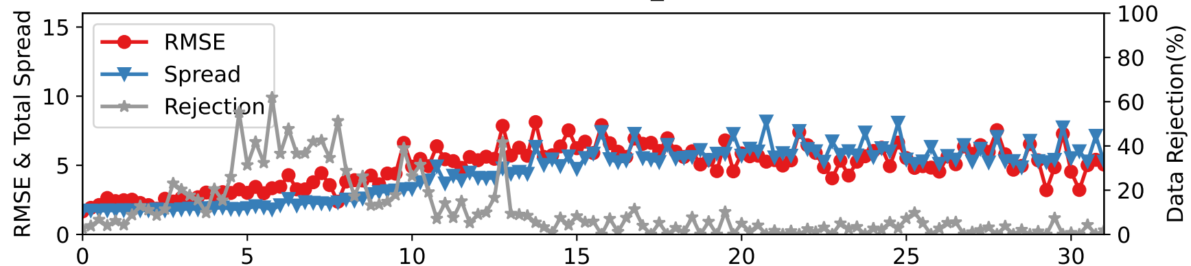
CTRLN10 — RADIOSONDE_V at 600-775 hPa
