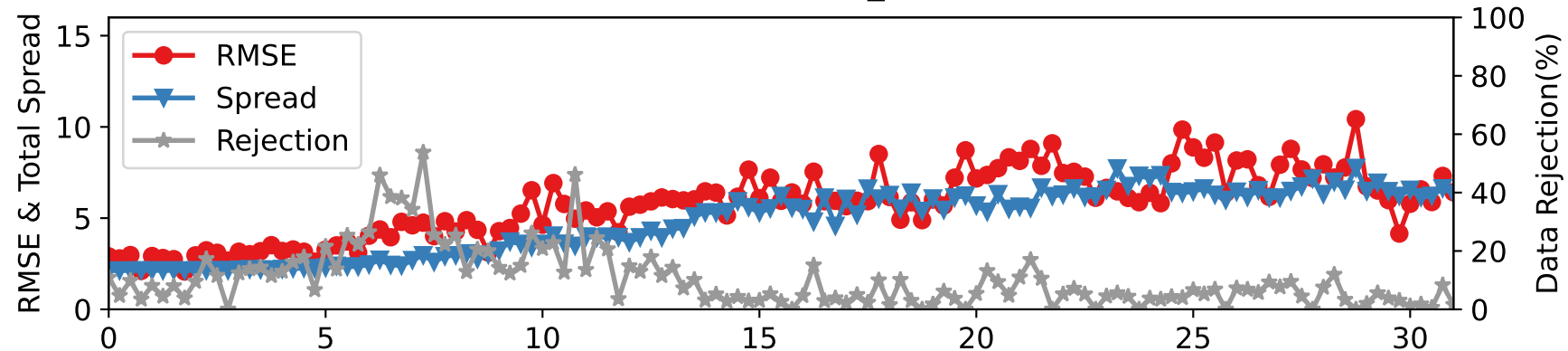
CTRLN10 — RADIOSONDE_V at 75-125 hPa
