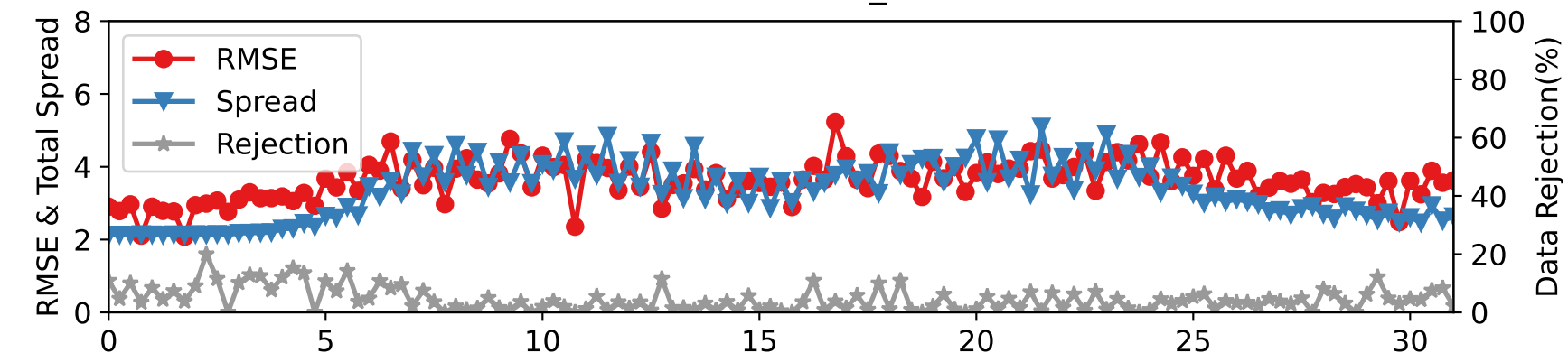
DARTEN20 — RADIOSONDE_V at 75-125 hPa
