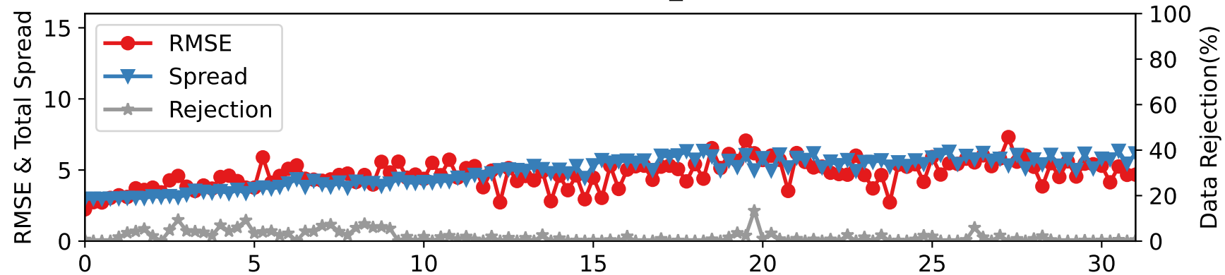
CTRLN10 — RADIOSONDE_V at 275-350 hPa
