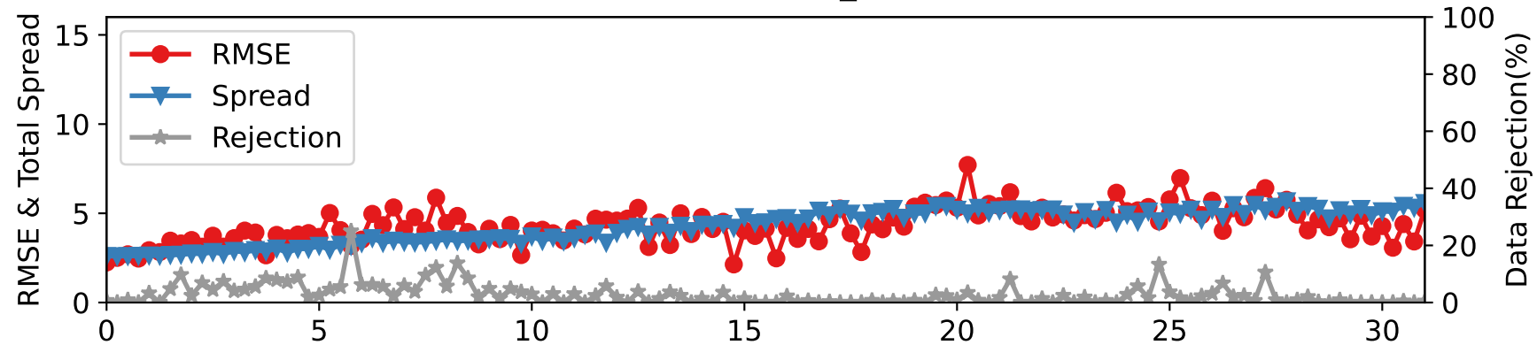
CTRLN10 — RADIOSONDE_V at 350-450 hPa
