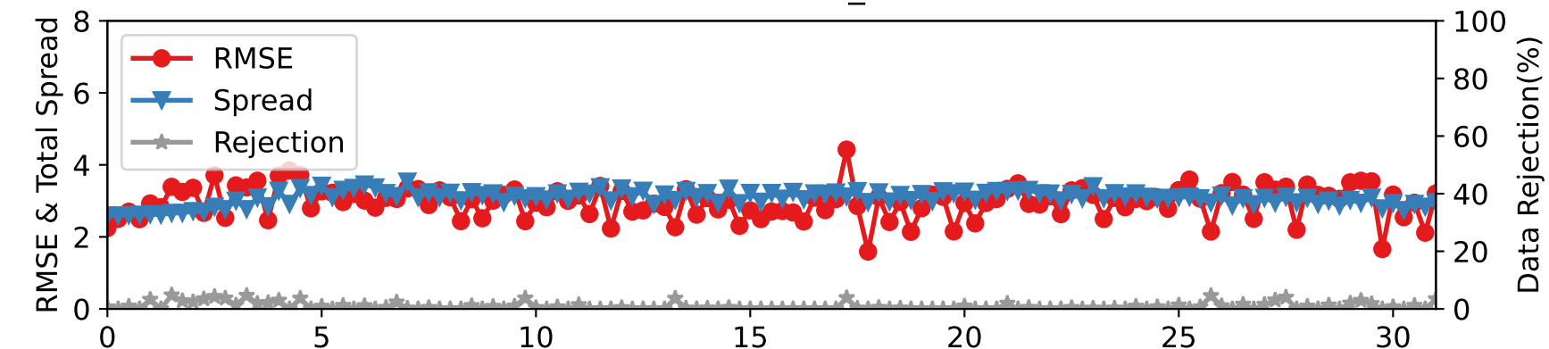
DARTEN20 — RADIOSONDE_V at 350-450 hPa
