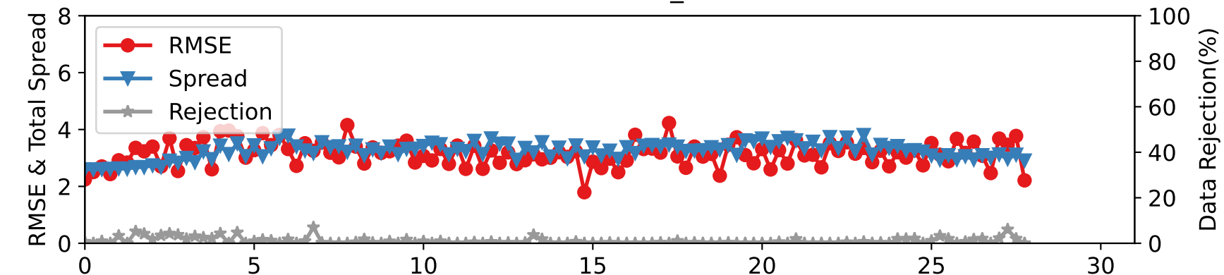
DARTEN10 — RADIOSONDE_V at 350-450 hPa
