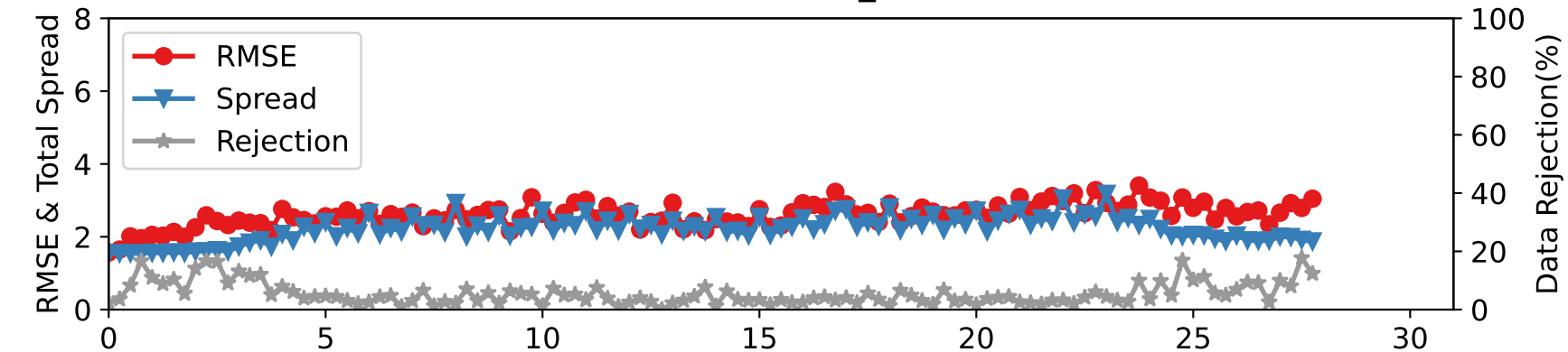
DARTEN10 — RADIOSONDE_V at 775-887 hPa
