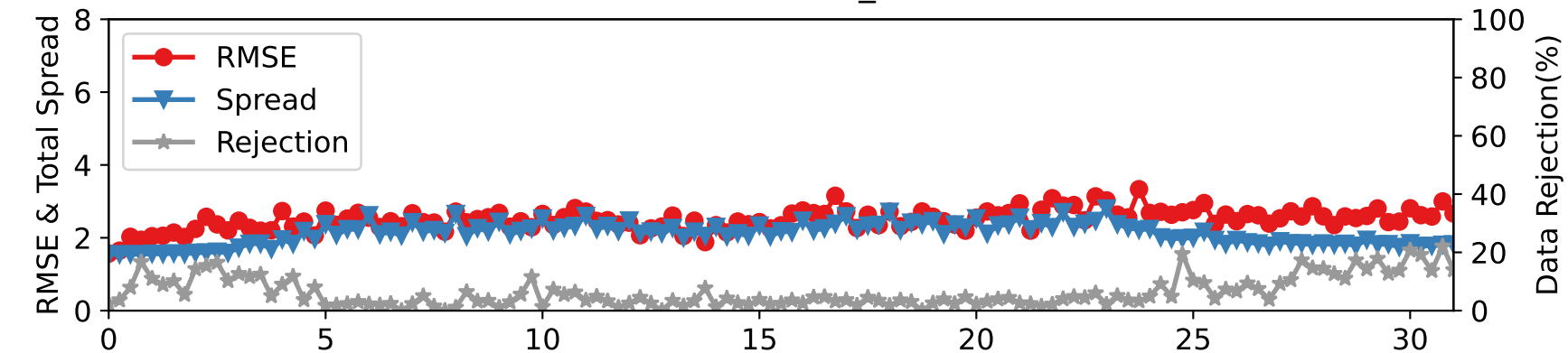
DARTEN20 — RADIOSONDE_V at 775-887 hPa
