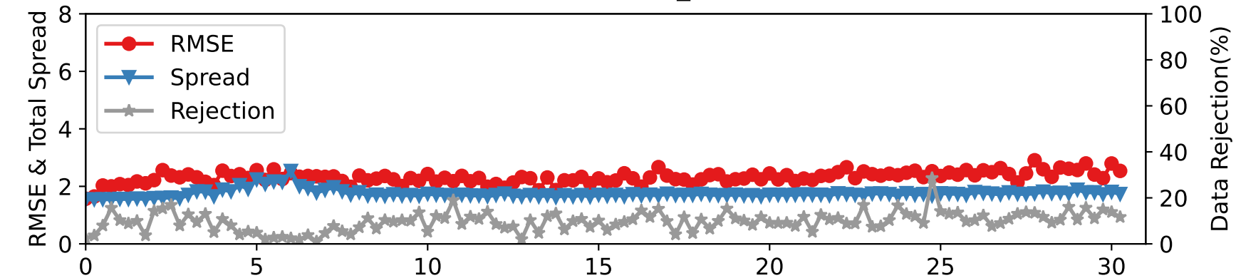
DARTEN40 — RADIOSONDE_V at 775-887 hPa
