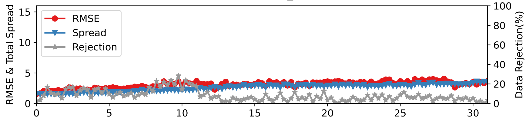
CTRLN10 — RADIOSONDE_V at 775-887 hPa
