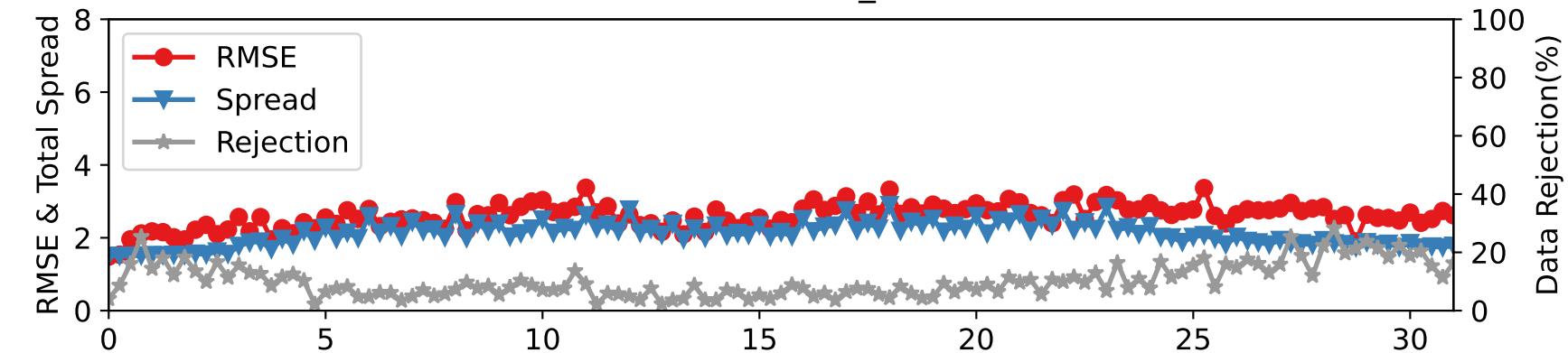
DARTEN20 — RADIOSONDE_V at 887-962 hPa
