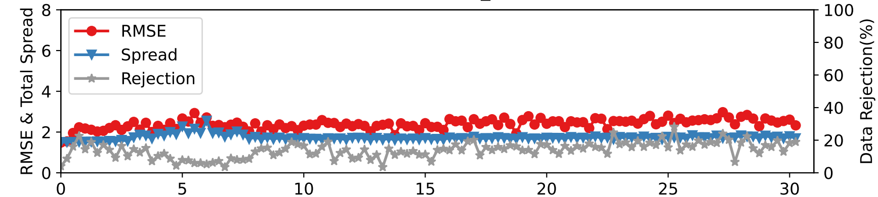
DARTEN40 — RADIOSONDE_V at 887-962 hPa
