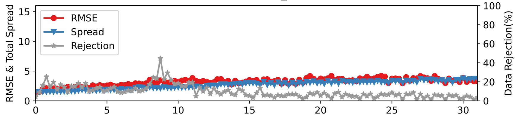
CTRLN10 — RADIOSONDE_V at 887-962 hPa
