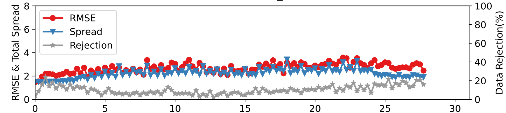
DARTEN10 — RADIOSONDE_V at 887-962 hPa
