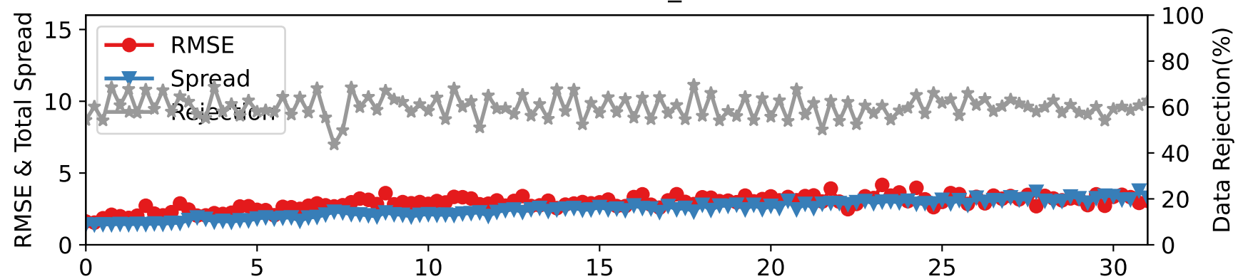
CTRLLEN10 — RADIOSONDE_V at 962-1035 hPa
