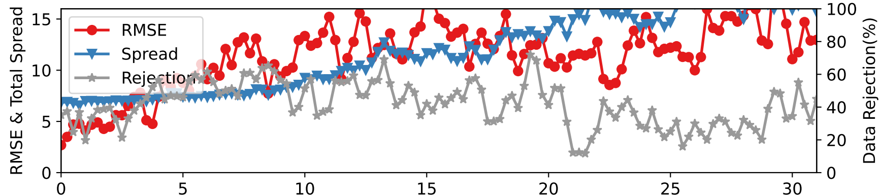
CTRLN10 — SAT_U at 175-225 hPa
