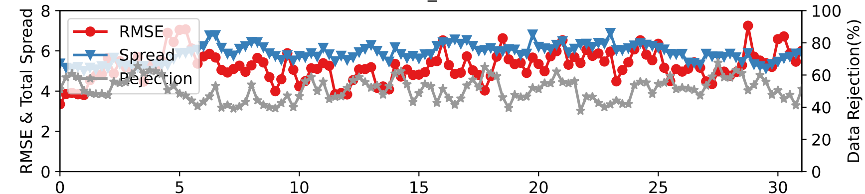
DARTEN20 — SAT_U at 350-450 hPa
