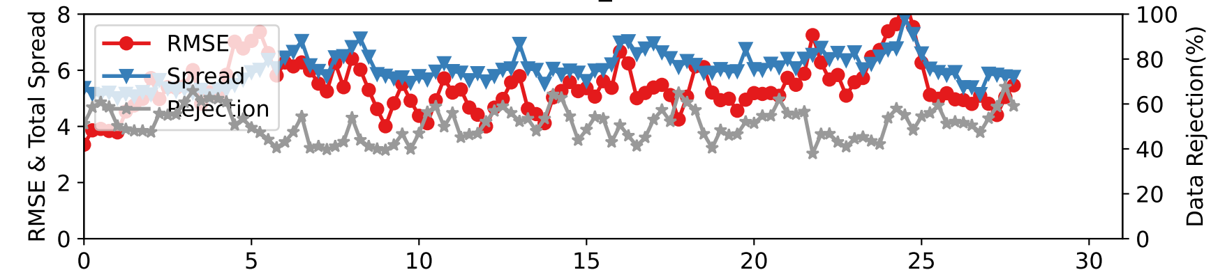
DARTEN10 — SAT_U at 350-450 hPa
