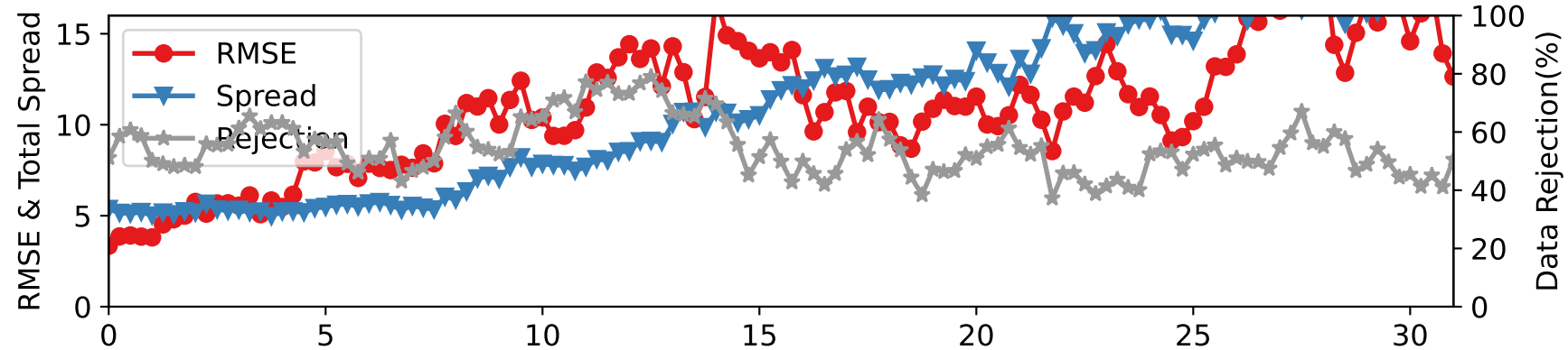
CTRLN10 — SAT_U at 350-450 hPa
