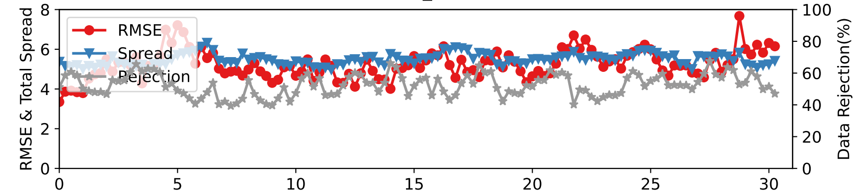
DARTEN40 — SAT_U at 350-450 hPa
