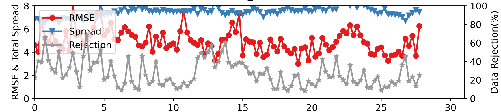
DARTEN10 — SAT_U at 125-175 hPa
