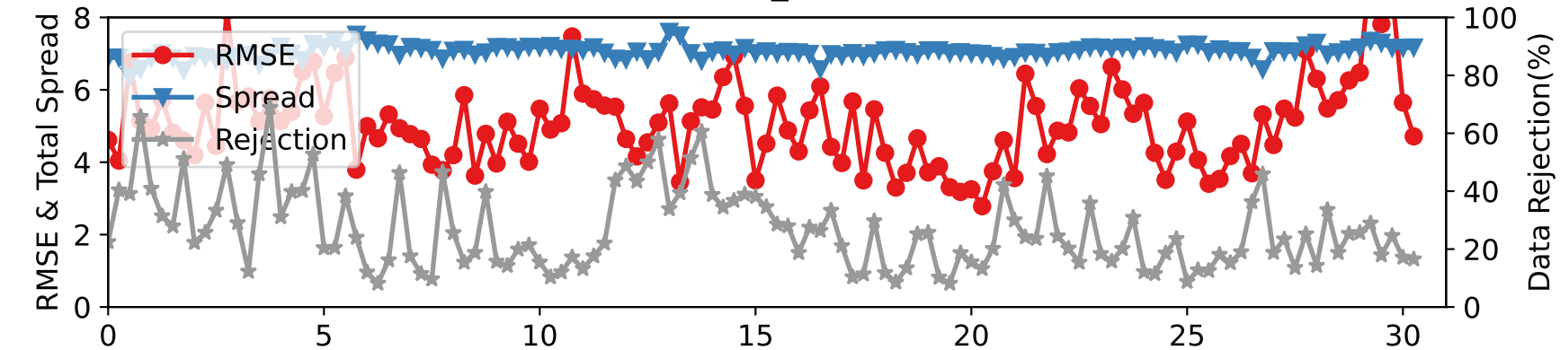
DARTEN40 — SAT_U at 125-175 hPa
