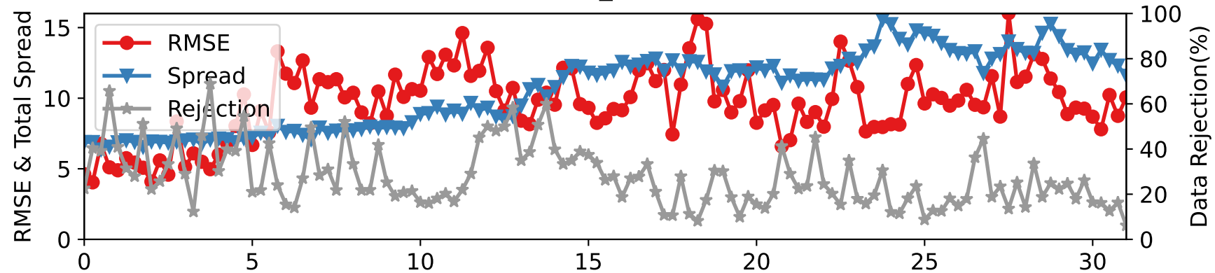
CTRLN10 — SAT_U at 125-175 hPa
