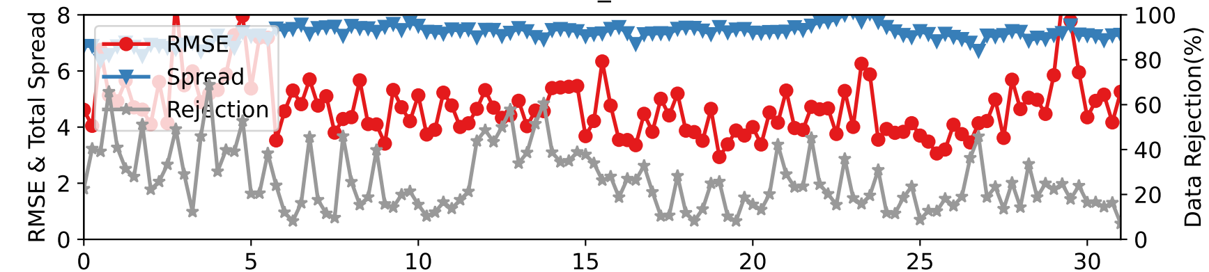
DARTEN20 — SAT_U at 125-175 hPa
