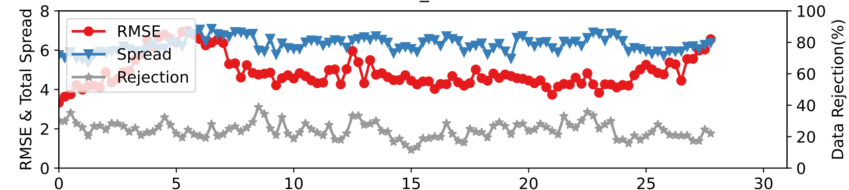
DARTEN10 — SAT_U at 275-350 hPa
