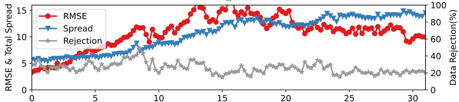
CTRLN10 — SAT_U at 275-350 hPa
