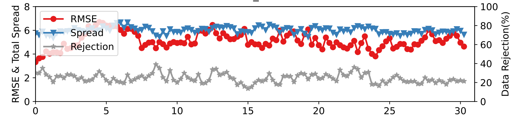
DARTEN40 — SAT_U at 275-350 hPa
