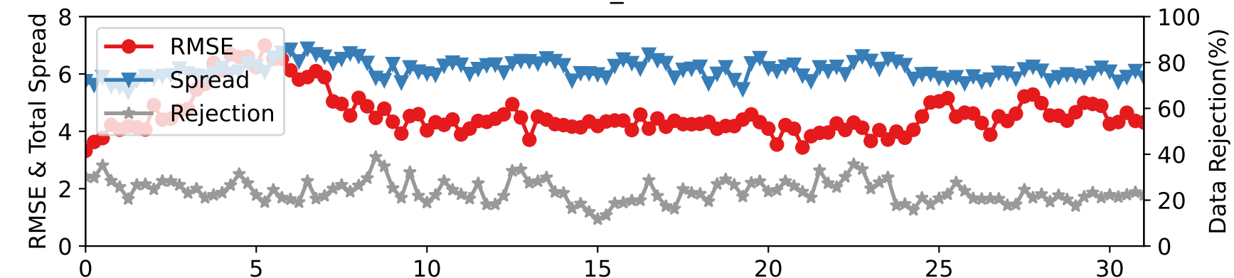
DARTEN20 — SAT_U at 275-350 hPa
