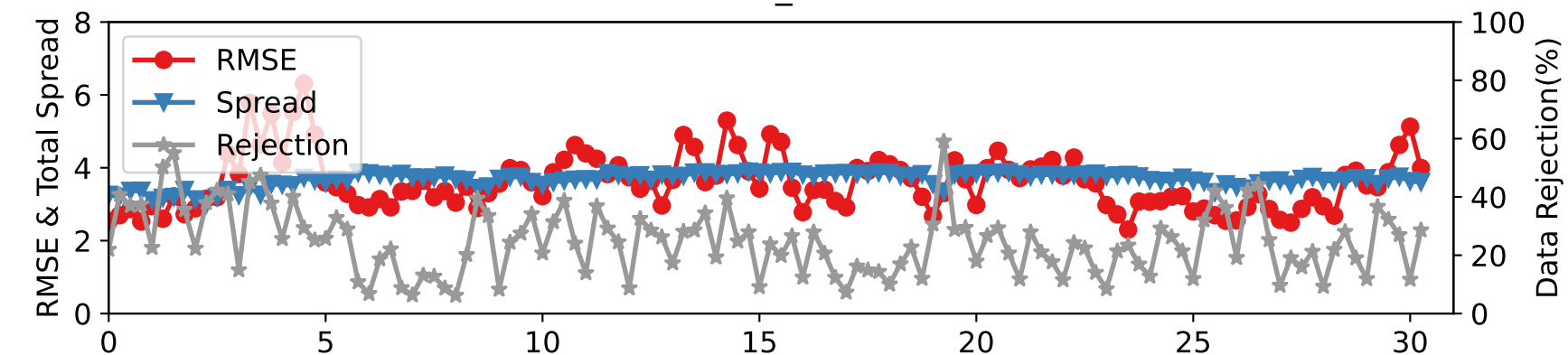
DARTEN40 — SAT_U at 600-775 hPa
