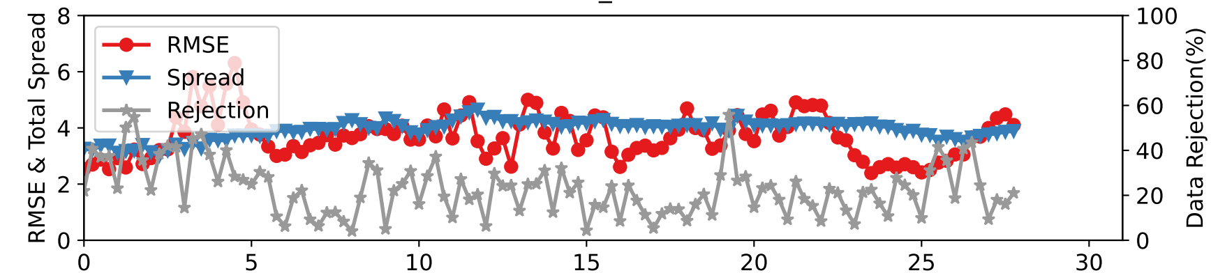
DARTEN10 — SAT_U at 600-775 hPa
