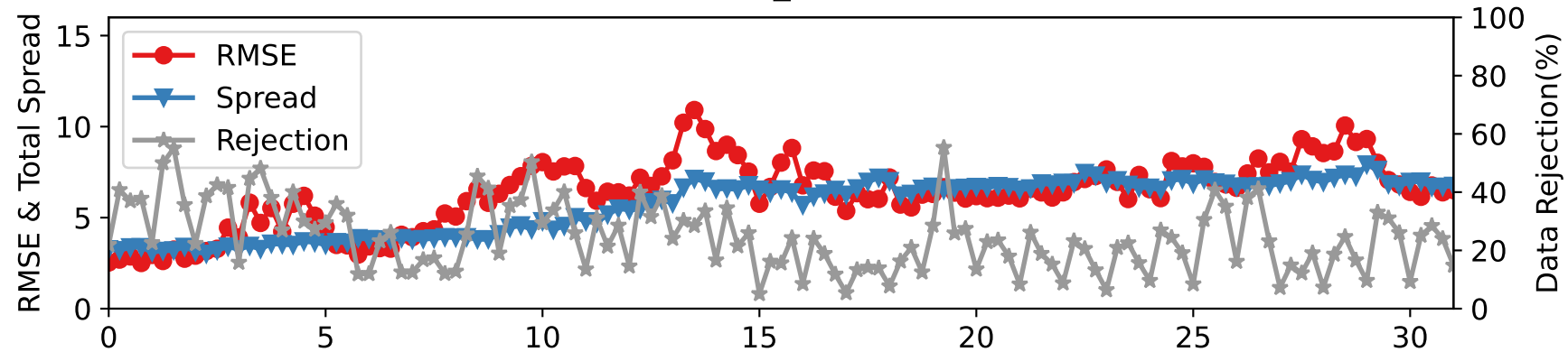
CTRLN10 — SAT_U at 600-775 hPa
