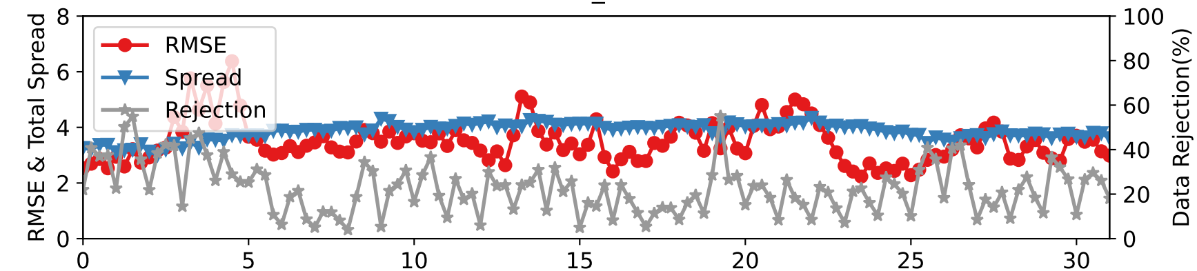
DARTEN20 — SAT_U at 600-775 hPa
