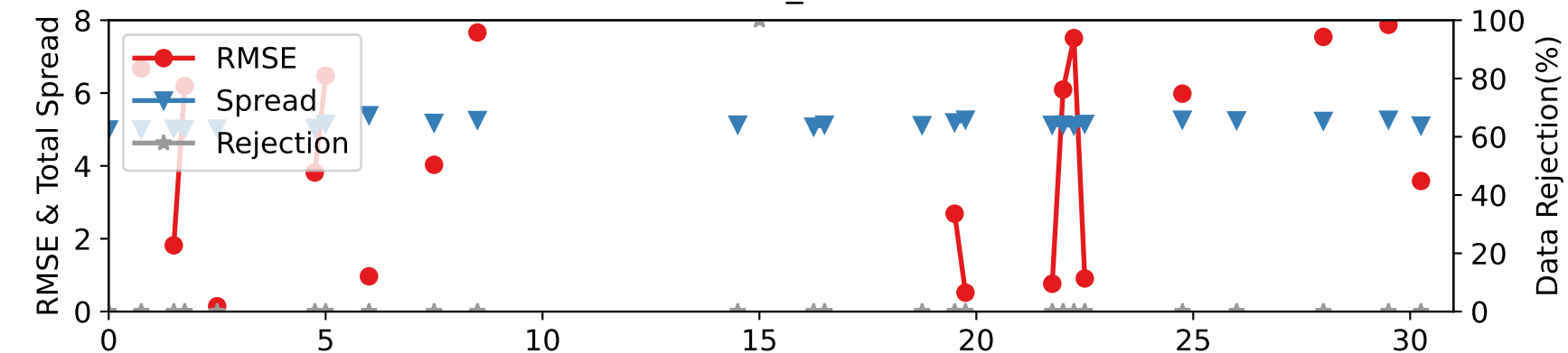
DARTEN40 — SAT_U at 75-125 hPa
