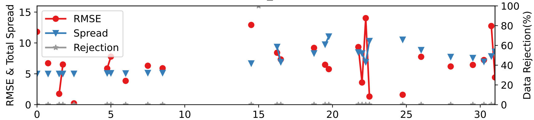
CTRLLEN10 — SAT_U at 75-125 hPa
