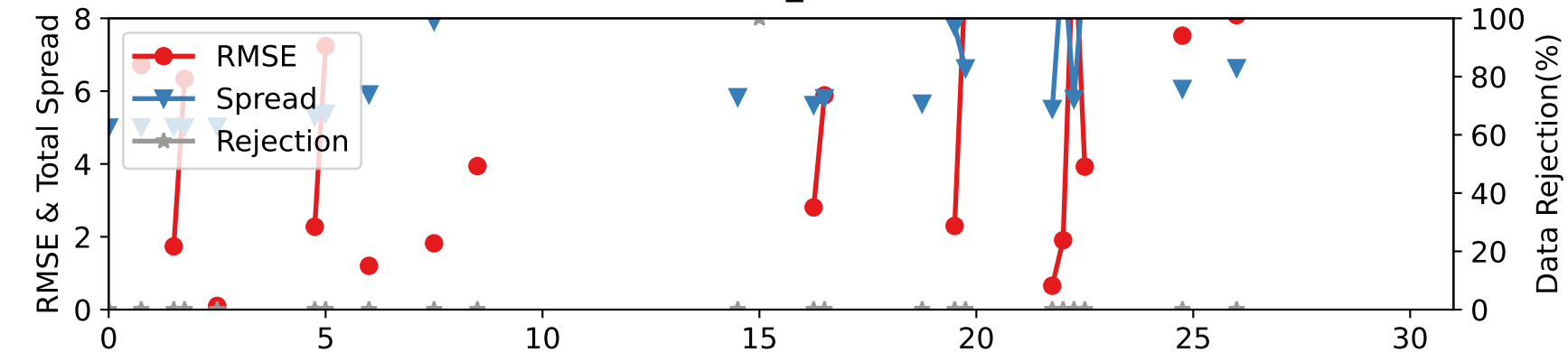
DARTEN10 — SAT_U at 75-125 hPa
