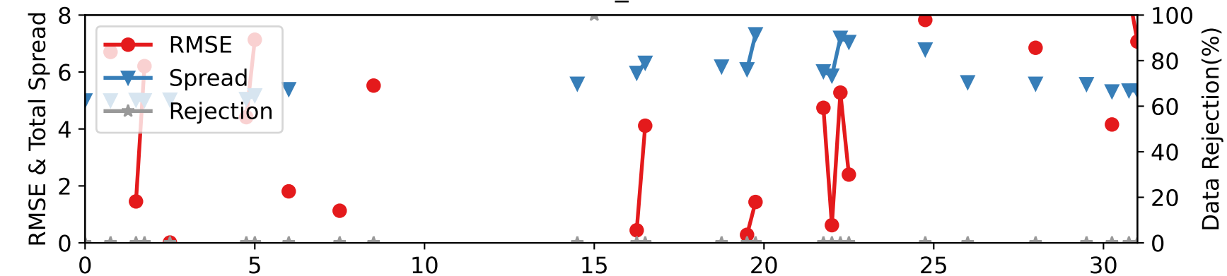
DARTEN20 — SAT_U at 75-125 hPa
