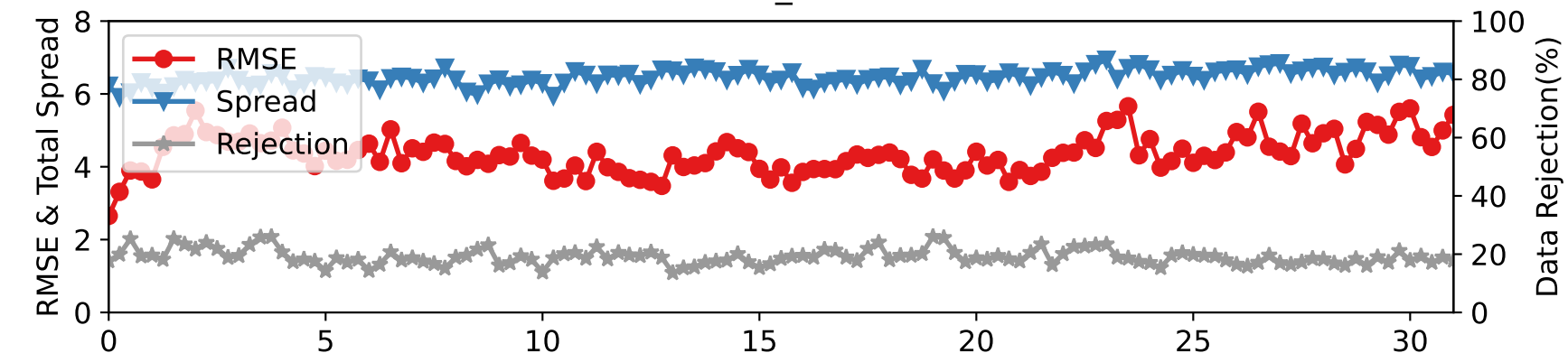
DARTEN20 — SAT_U at 225-275 hPa
