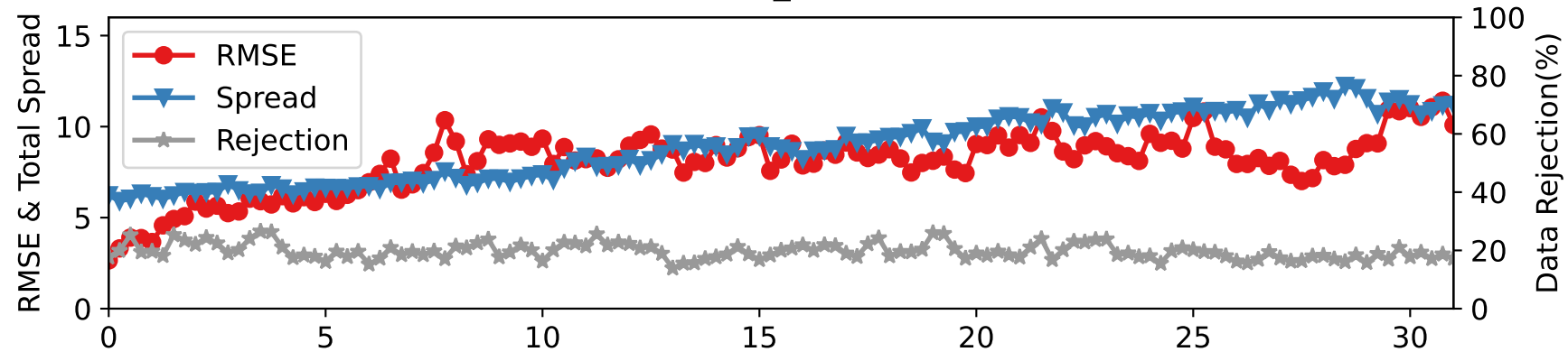
CTRLN10 — SAT_U at 225-275 hPa
