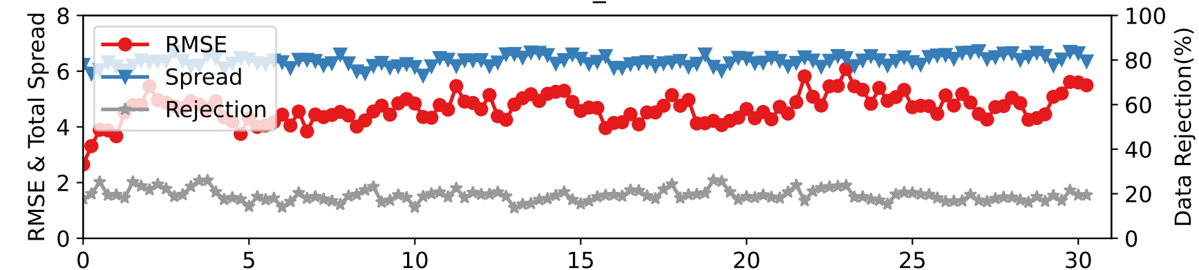
DARTEN40 — SAT_U at 225-275 hPa
