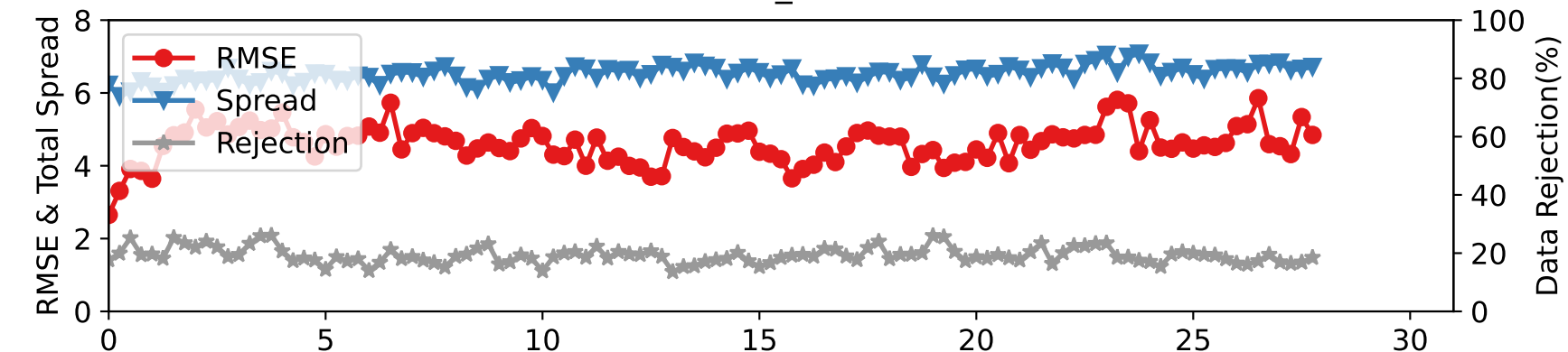
DARTEN10 — SAT_U at 225-275 hPa
