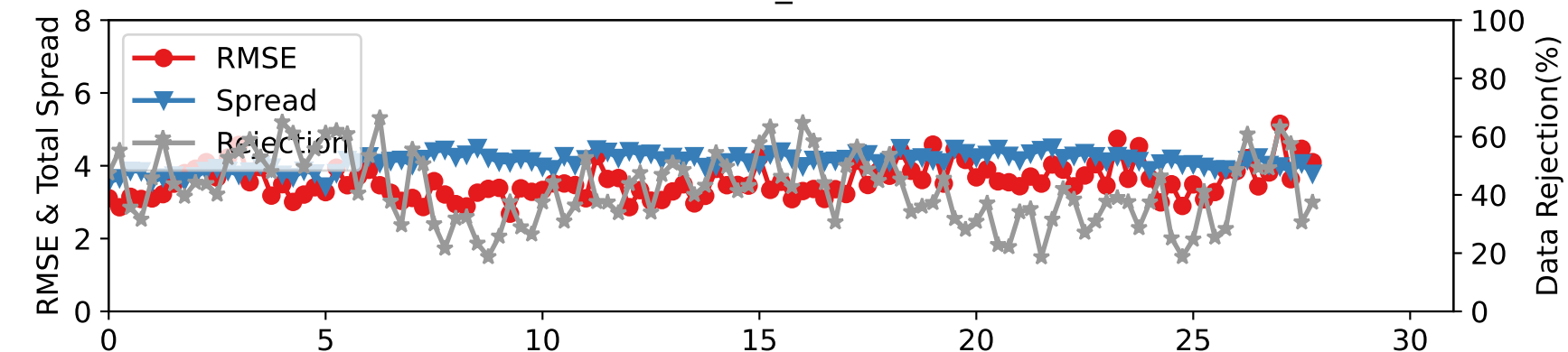
DARTEN10 — SAT_U at 450-600 hPa
