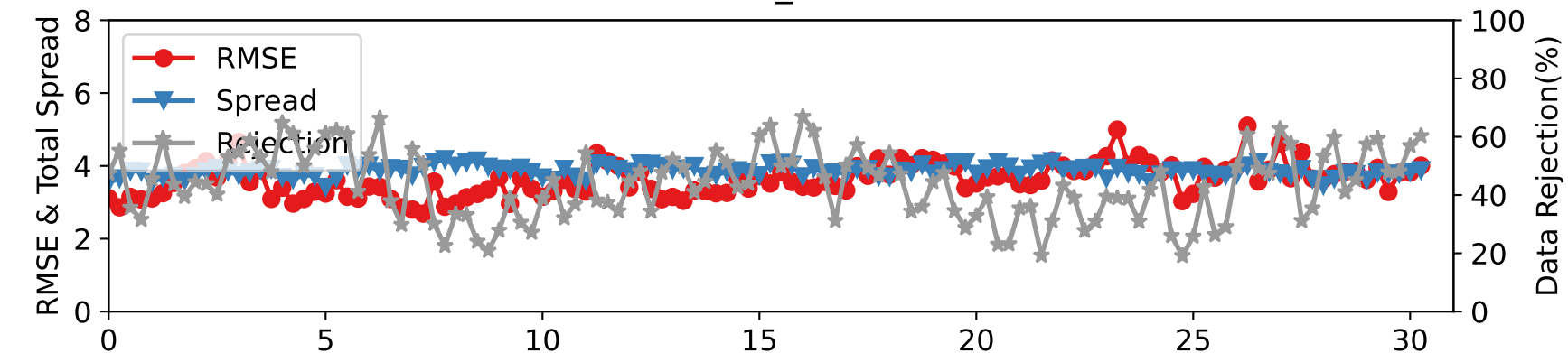
DARTEN40 — SAT_U at 450-600 hPa
