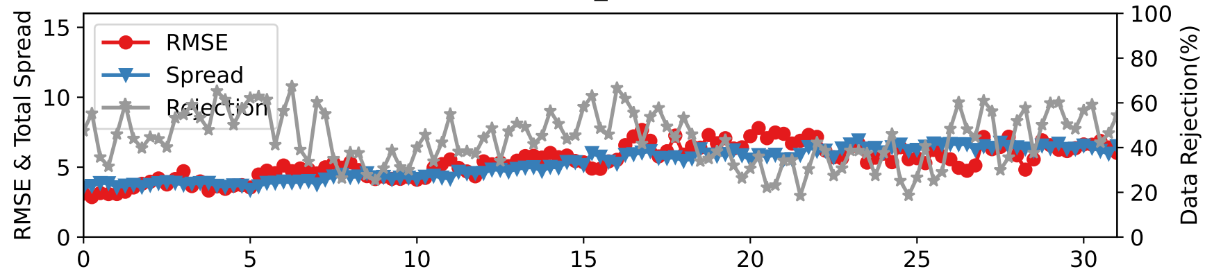
CTRLN10 — SAT_U at 450-600 hPa
