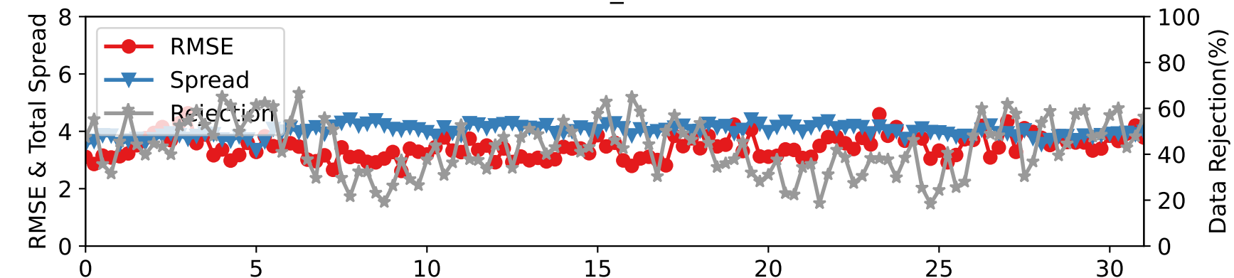
DARTEN20 — SAT_U at 450-600 hPa
