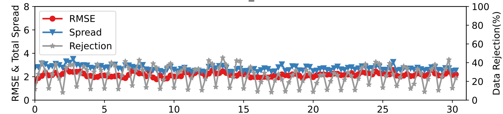
DARTEN40 — SAT_U at 775-887 hPa
