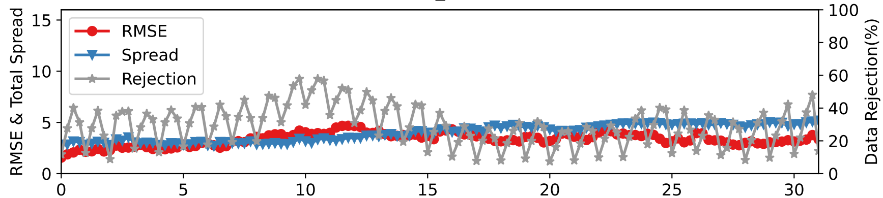
CTRLN10 — SAT_U at 775-887 hPa
