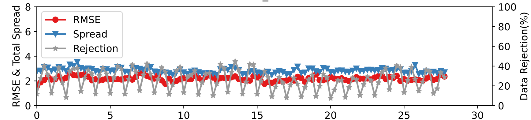
DARTEN10 — SAT_U at 775-887 hPa
