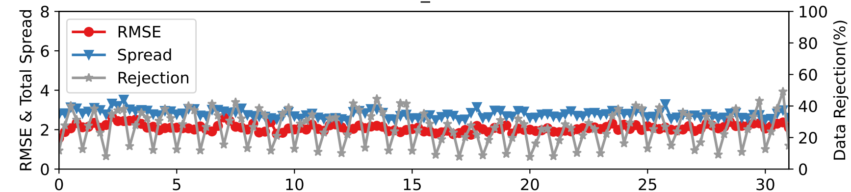
DARTEN20 — SAT_U at 775-887 hPa
