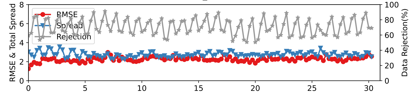
DARTEN40 — SAT_U at 887-962 hPa
