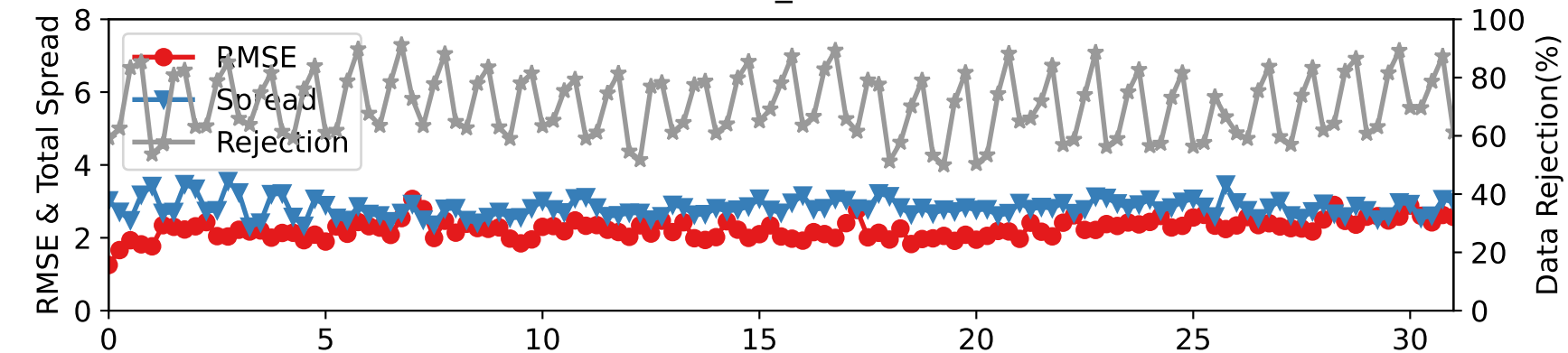
DARTEN20 — SAT_U at 887-962 hPa
