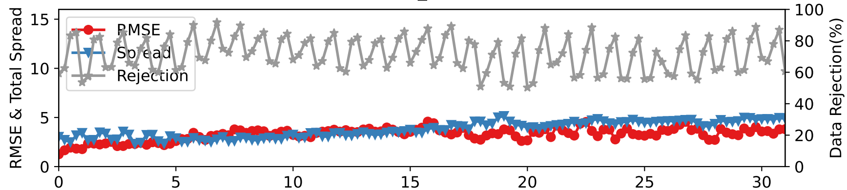
CTRLN10 — SAT_U at 887-962 hPa
