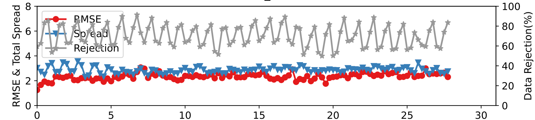
DARTEN10 — SAT_U at 887-962 hPa
