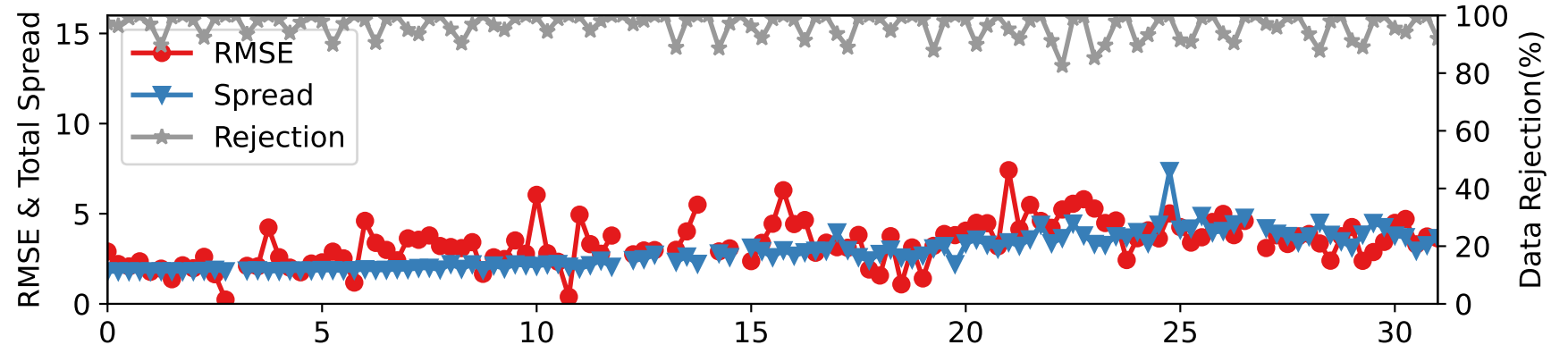
CTRLN10 — SAT_U at 962-1035 hPa
