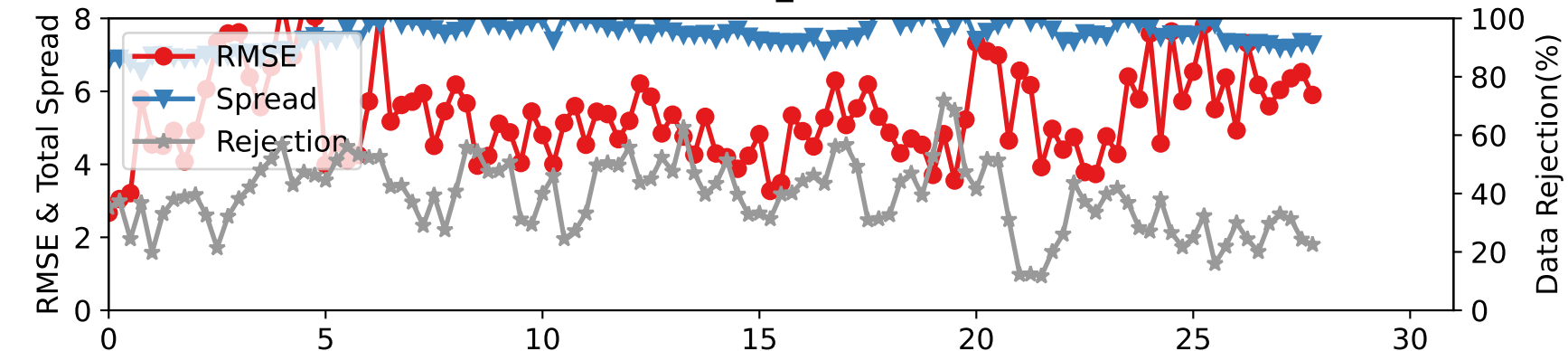
DARTEN10 — SAT_V at 175-225 hPa
