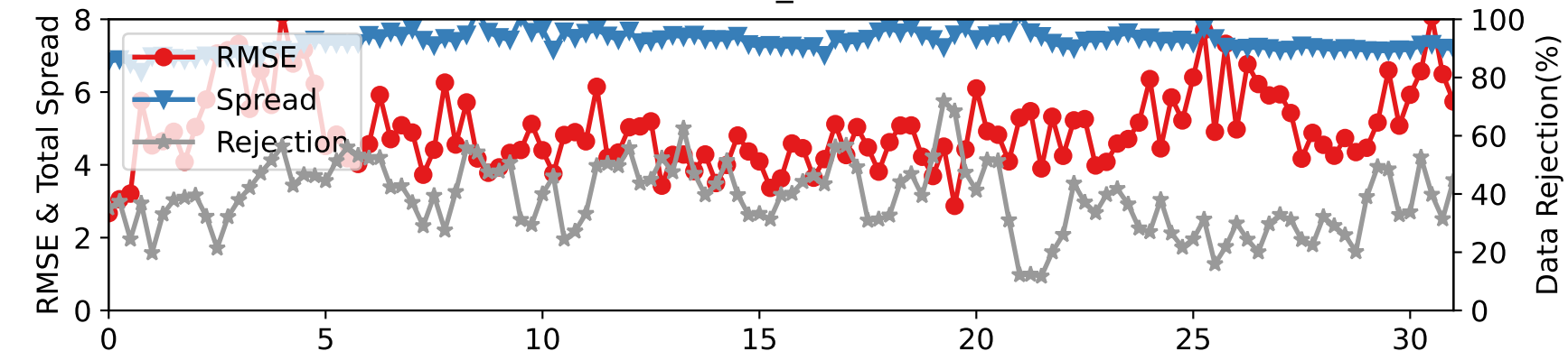
DARTEN20 — SAT_V at 175-225 hPa
