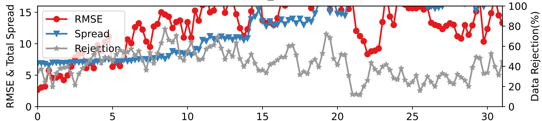
CTRLN10 — SAT_V at 175-225 hPa
