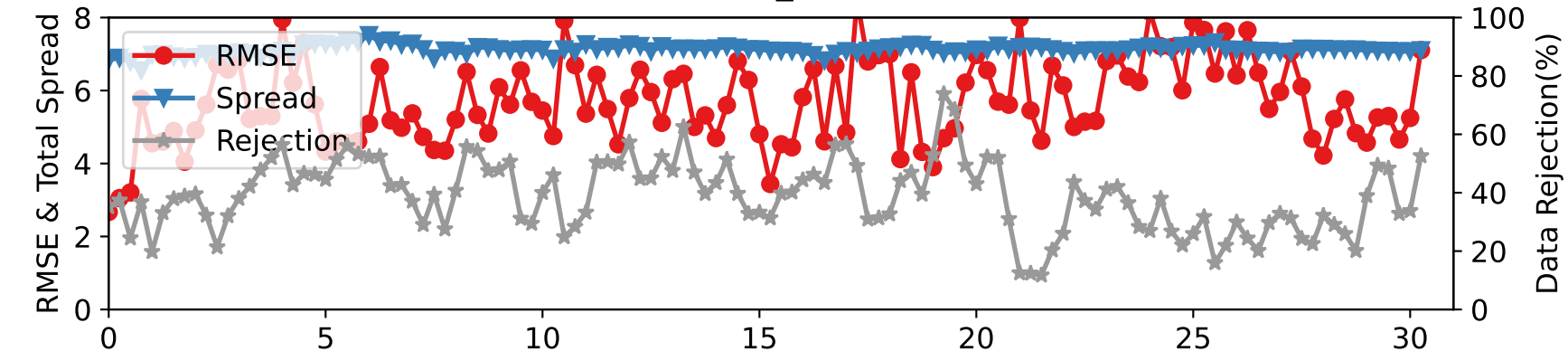
DARTEN40 — SAT_V at 175-225 hPa
