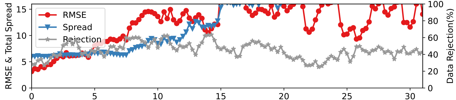
CTRLN10 — SAT_V at 275-350 hPa
