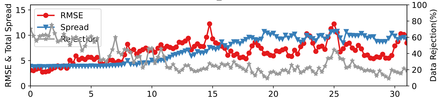
CTRLN10 — SAT_V at 600-775 hPa
