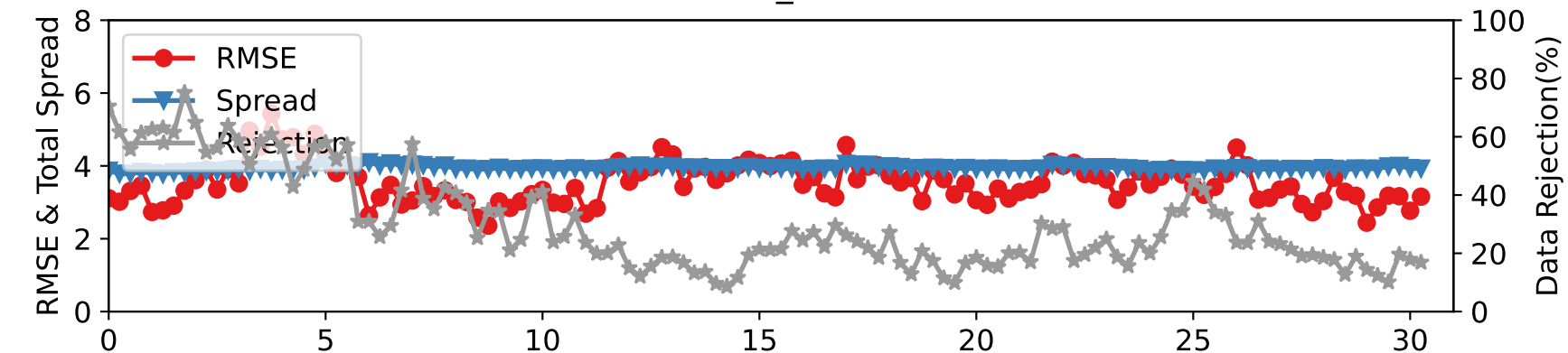
DARTEN40 — SAT_V at 600-775 hPa
