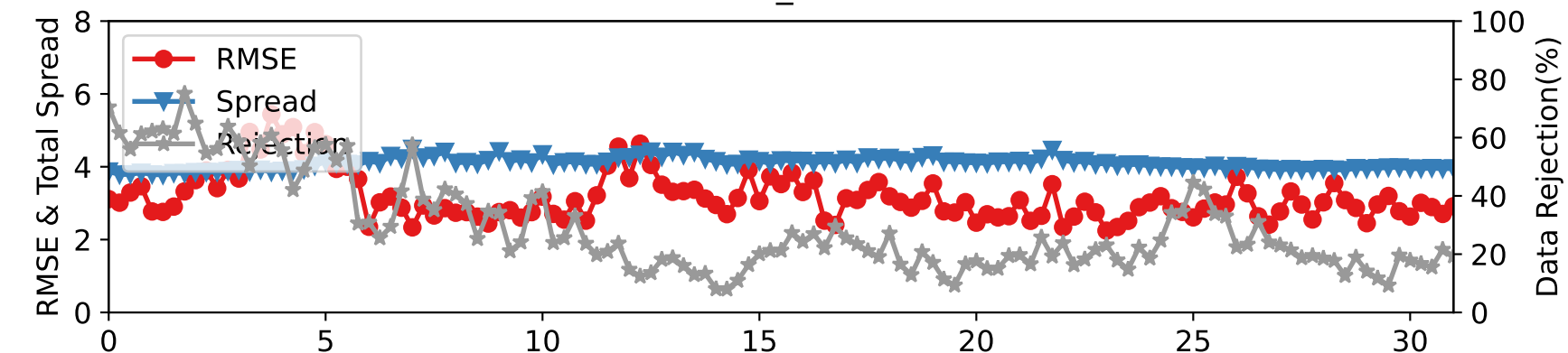
DARTEN20 — SAT_V at 600-775 hPa
