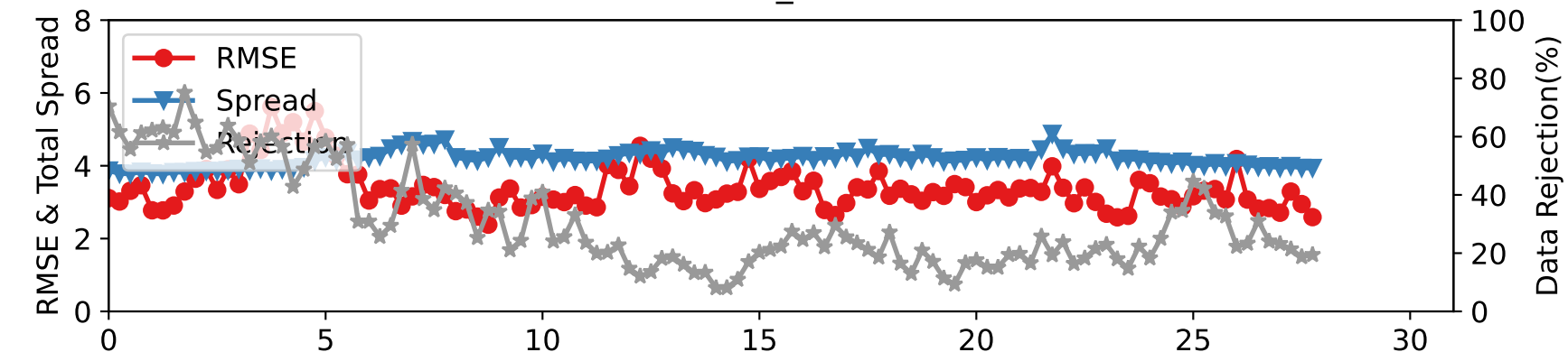
DARTEN10 — SAT_V at 600-775 hPa
