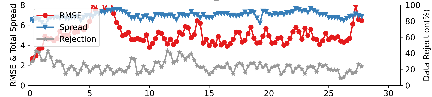
DARTEN10 — SAT_V at 225-275 hPa
