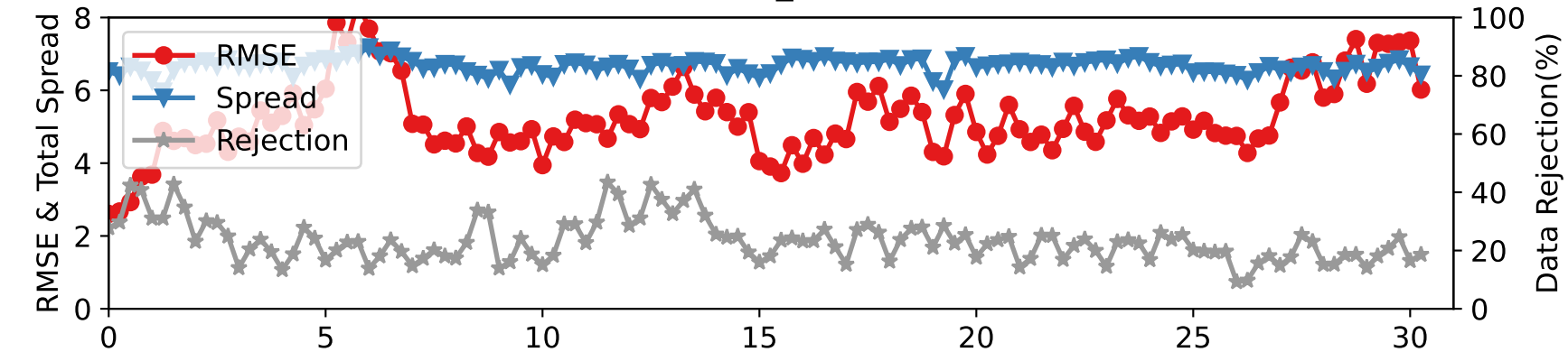
DARTEN40 — SAT_V at 225-275 hPa
