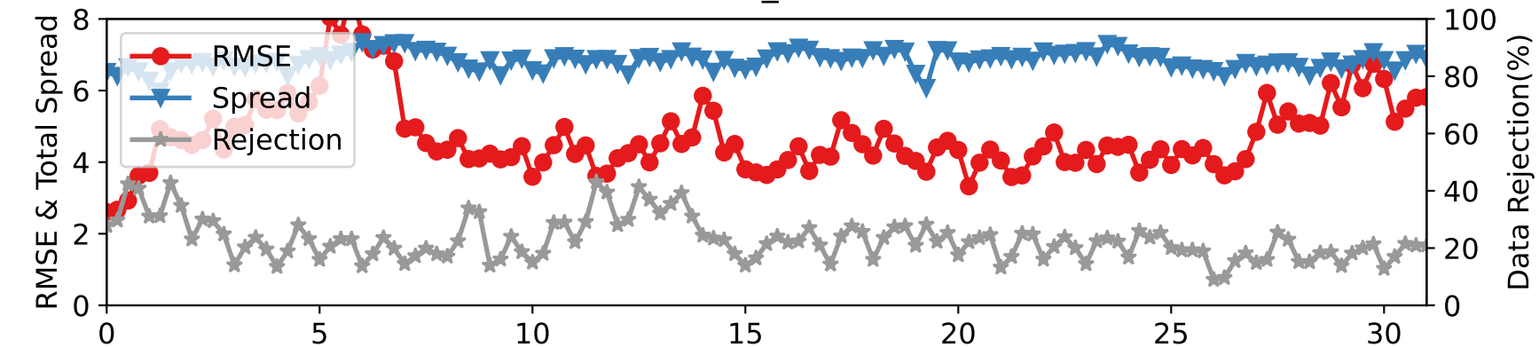
DARTEN20 — SAT_V at 225-275 hPa
