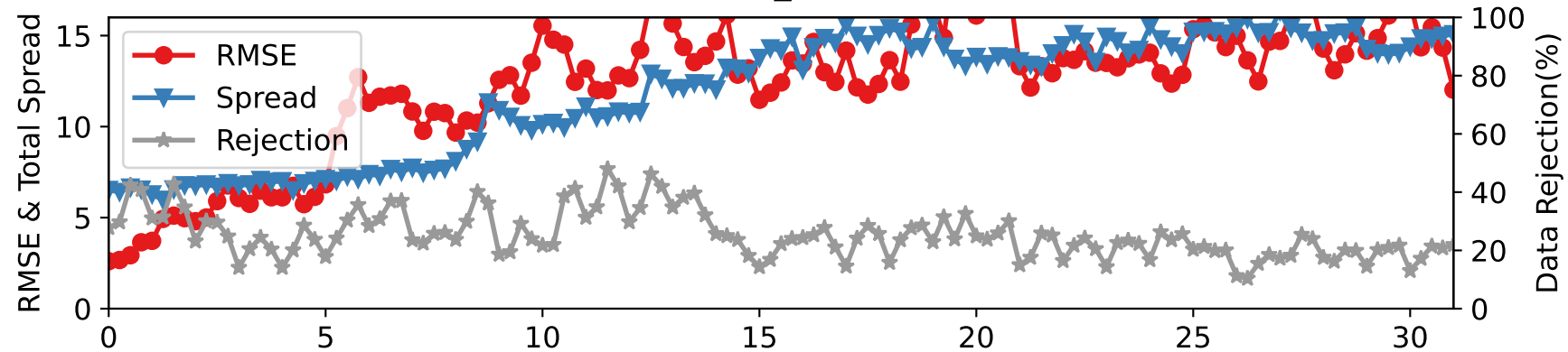
CTRLN10 — SAT_V at 225-275 hPa
