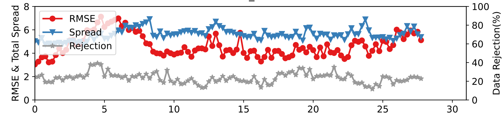
DARTEN10 — SAT_V at 350-450 hPa
