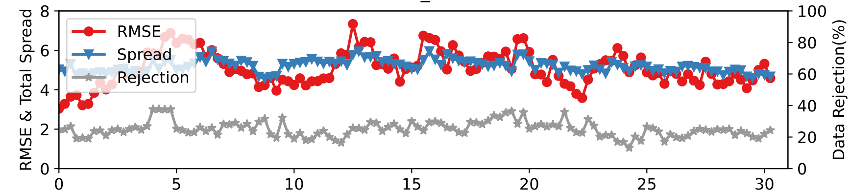
DARTEN40 — SAT_V at 350-450 hPa
