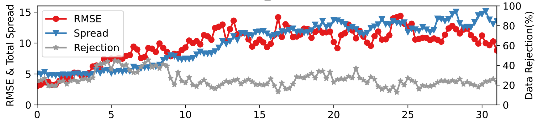
CTRLN10 — SAT_V at 350-450 hPa
