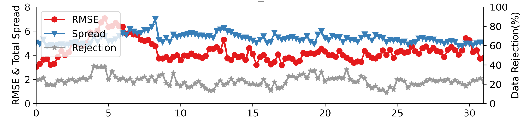
DARTEN20 — SAT_V at 350-450 hPa
