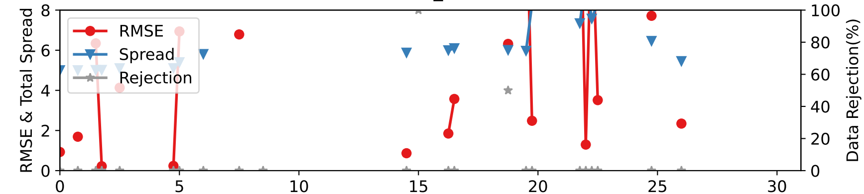
DARTEN10 — SAT_V at 75-125 hPa
