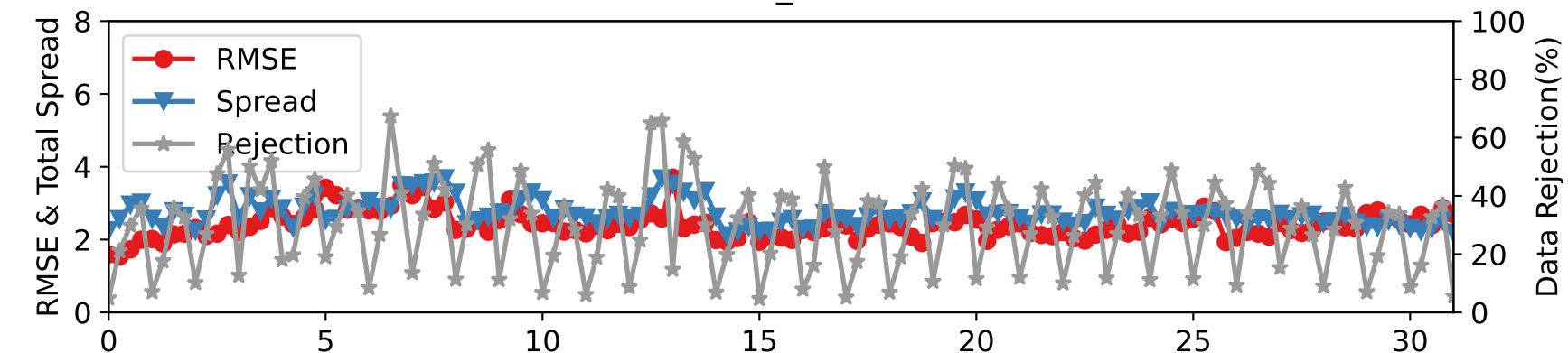
DARTEN20 — SAT_V at 775-887 hPa
