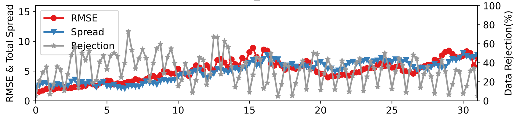
CTRLN10 — SAT_V at 775-887 hPa
