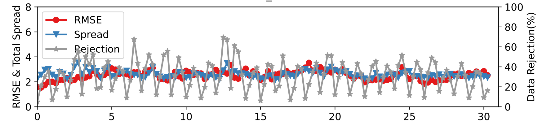
DARTEN40 — SAT_V at 775-887 hPa
