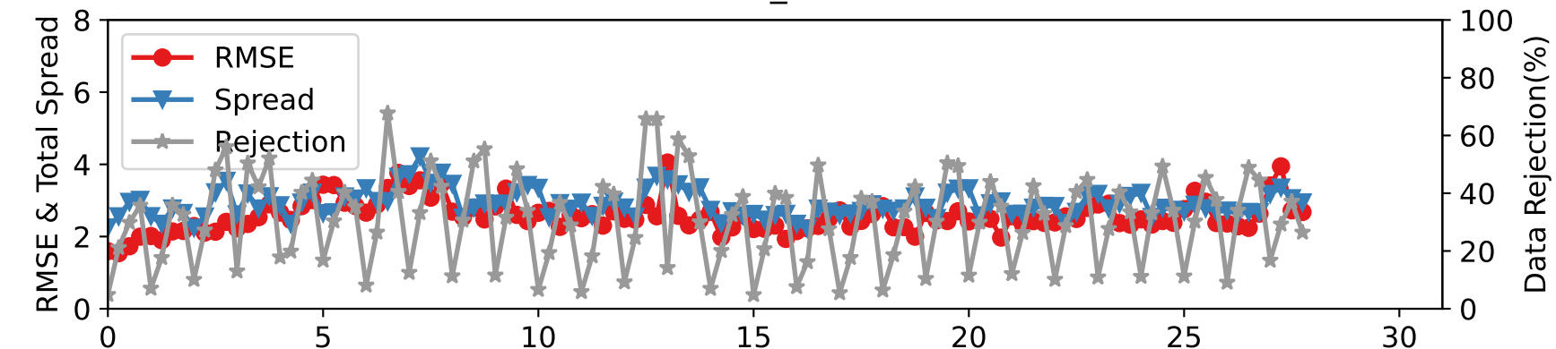
DARTEN10 — SAT_V at 775-887 hPa
