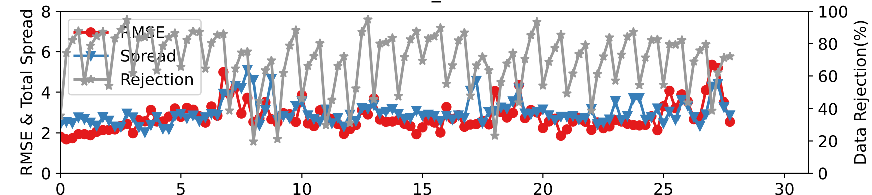
DARTEN10 — SAT_V at 887-962 hPa
