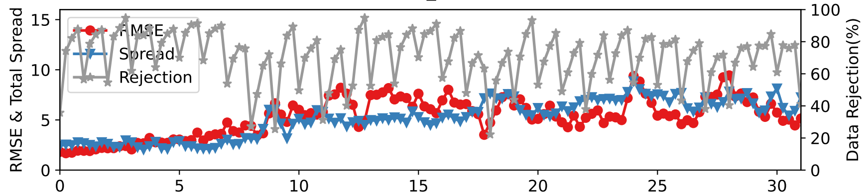
CTRLN10 — SAT_V at 887-962 hPa
