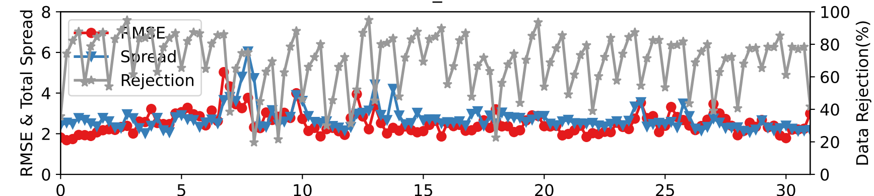
DARTEN20 — SAT_V at 887-962 hPa
