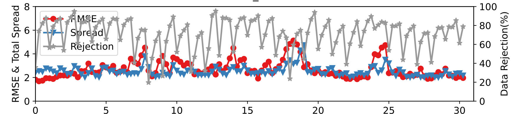
DARTEN40 — SAT_V at 887-962 hPa
