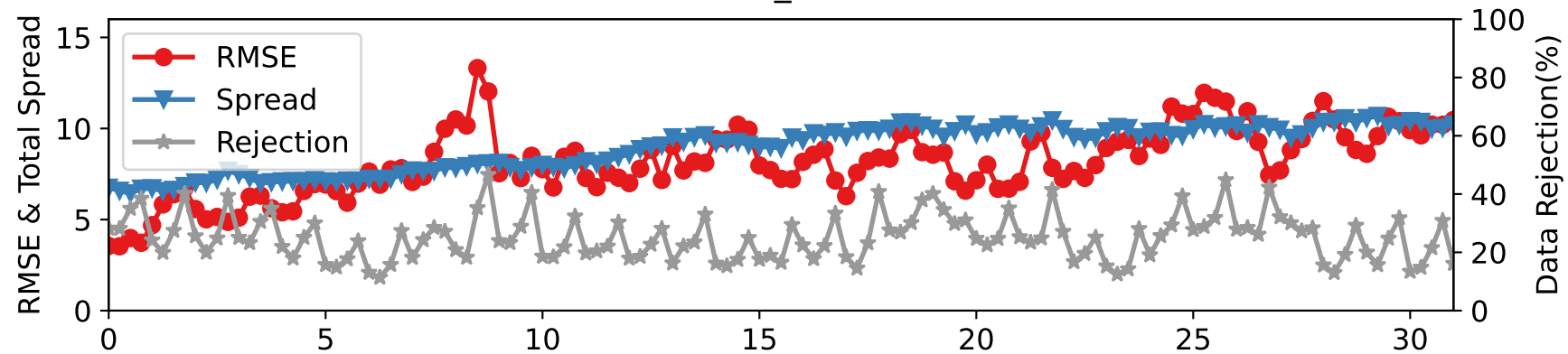
CTRLN10 — SAT_V at 125-175 hPa
