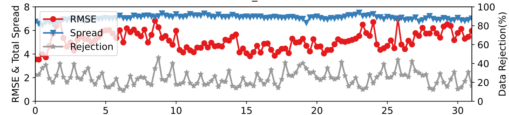
DARTEN20 — SAT_V at 125-175 hPa
