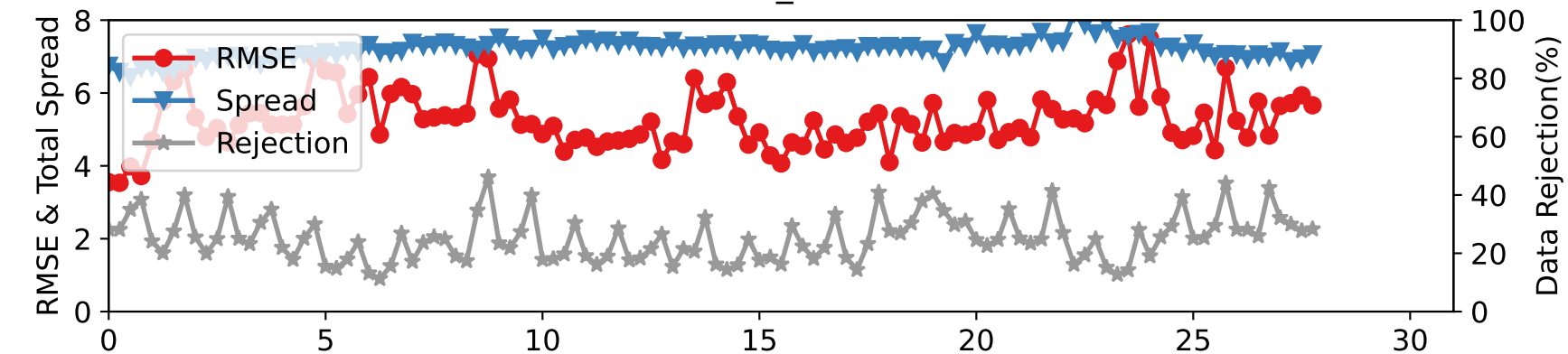
DARTEN10 — SAT_V at 125-175 hPa
