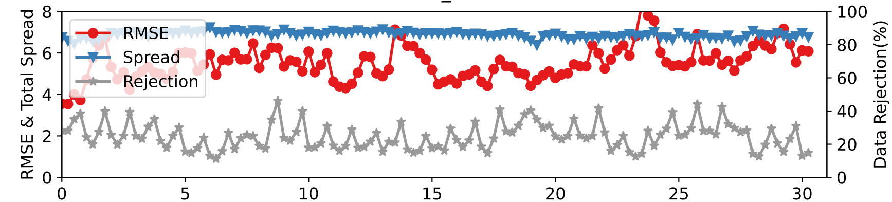
DARTEN40 — SAT_V at 125-175 hPa
