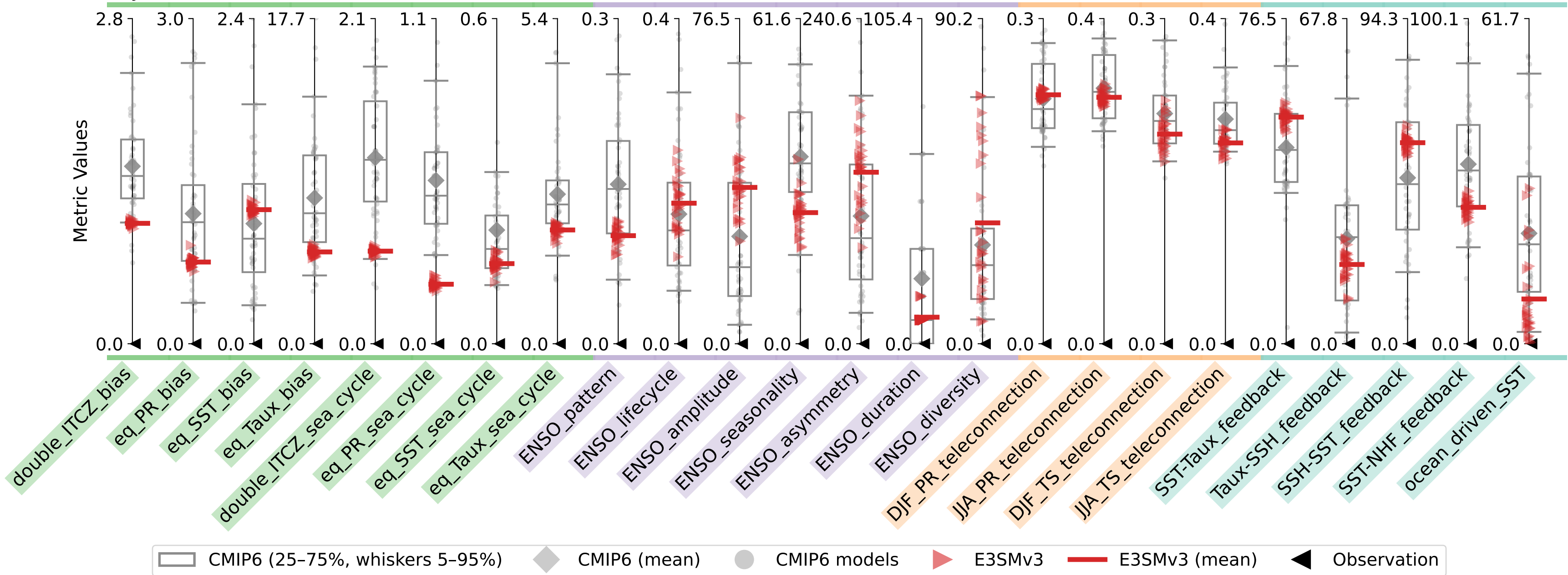
Key ENSO metrics (E3SMv3 versus CMIP6)
