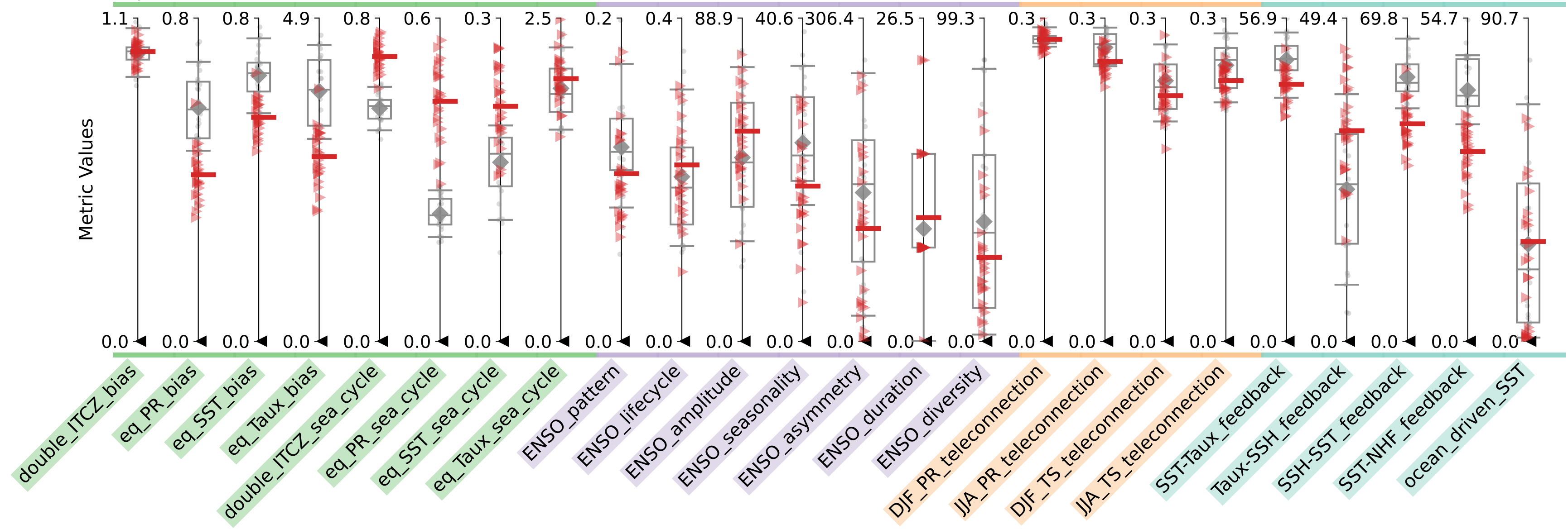
Key ENSO metrics (E3SMv3 historical versus near-future)
