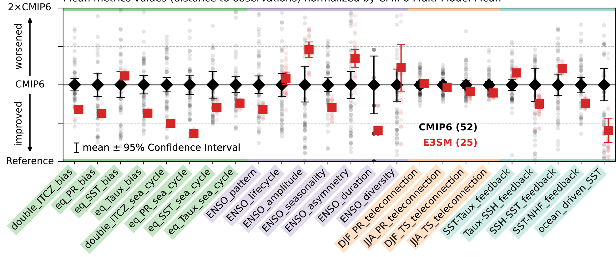
Mean metrics values (distance to observations) normalized by CMIP6 Multi-Model Mean
