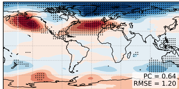
(b) LR NAO (DJF,1985-2014)
