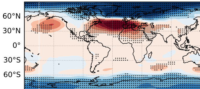
(a) obs NAO (DJF,1985-2014)
