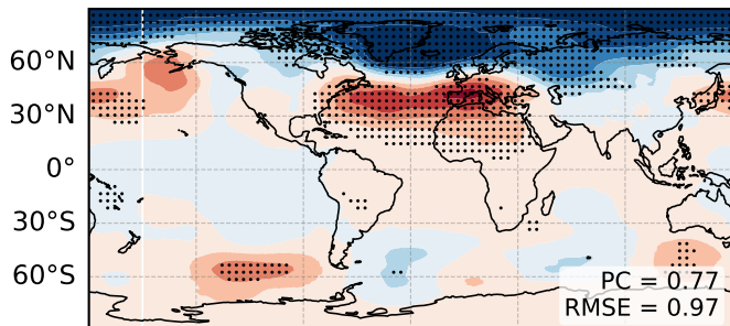
(e) EARRM NAO (DJF,1985-2014)
