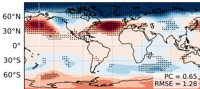
(c) NARRM NAO (DJF,1985-2014)
