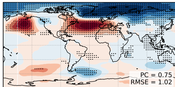
(f) AMZRRM NAO (DJF,1985-2014)
